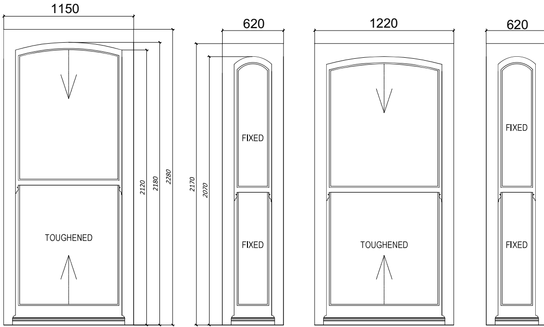
W-03 279_FLAT B FRONT WINDOW SLIMLINE / 14mm GLAZING / 4mm/6mm/4mm
