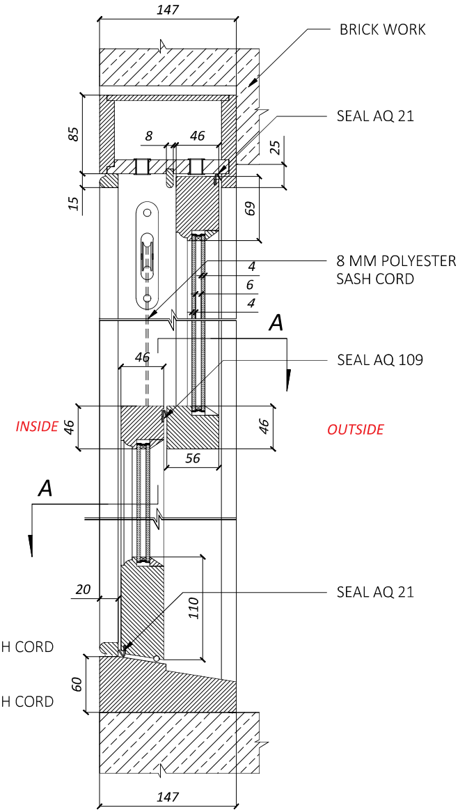
DETAIL 1 / 14 mm GLAZING SCALE 1:4
