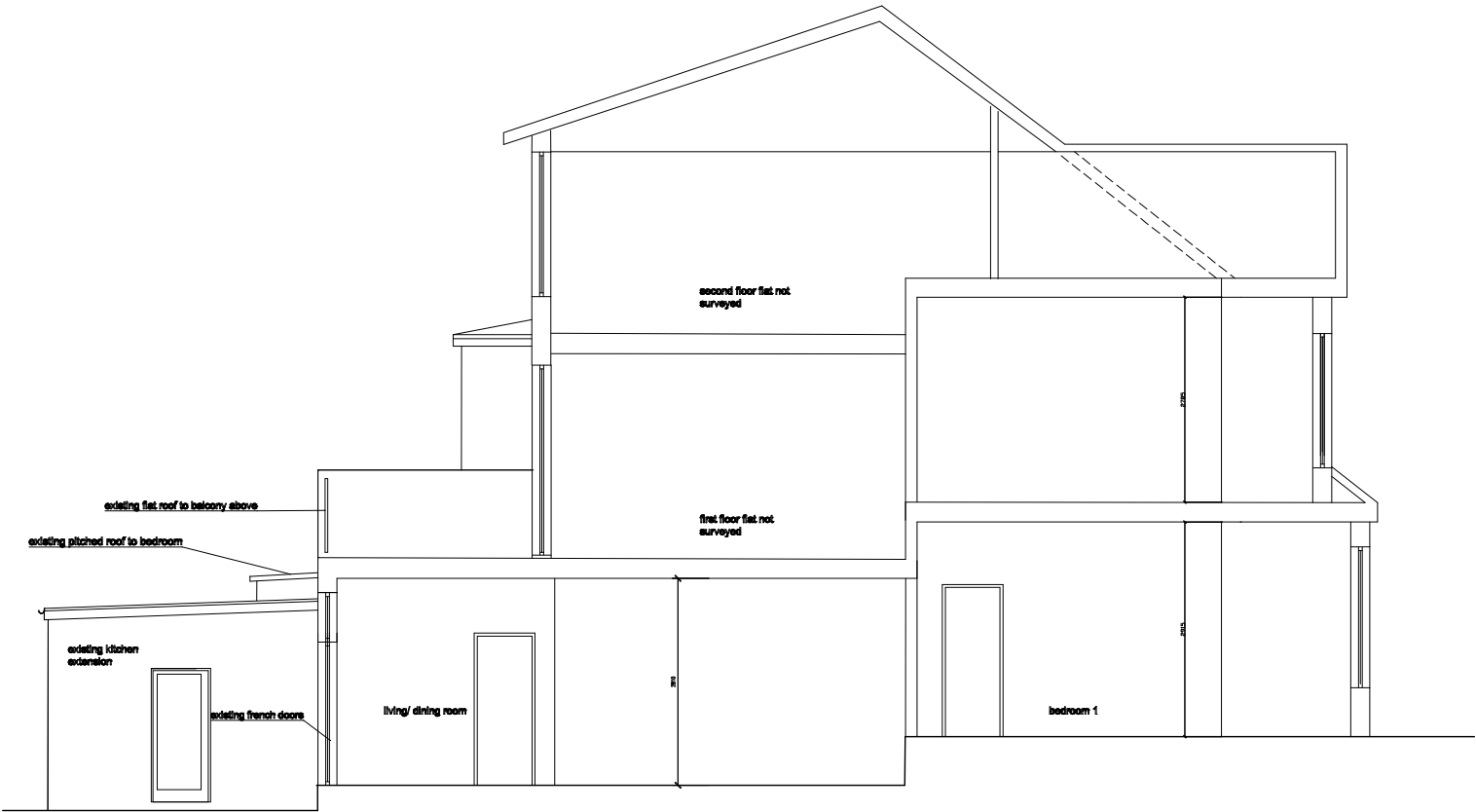
Existing section
