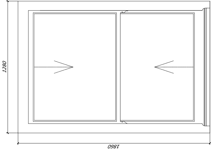
W-09 279_FLAT C / KITCHEN / BACK 24mm GLAZING / 4mm / 16mm / 4mm
