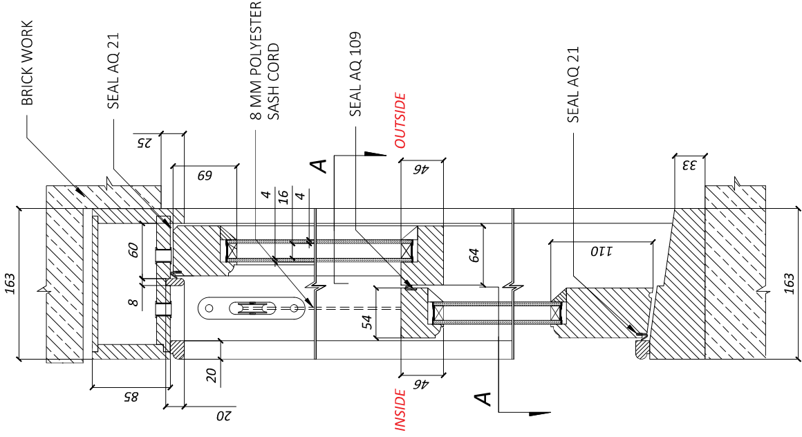
DETAIL 1 / 24 mm GLAZING SCALE 1:4
