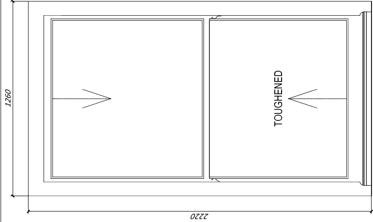
W-11 279_FLAT B 24mm GLAZING / 4mm / 16mm / 4mm
