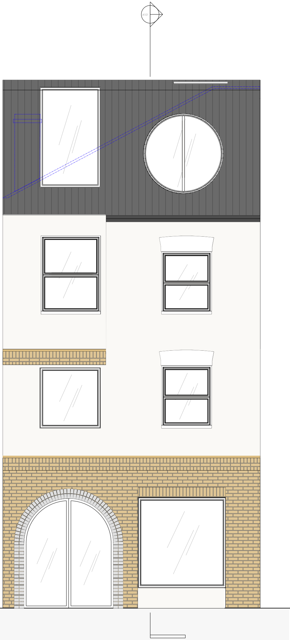
3 Proposed East Elevation 1 : 50
