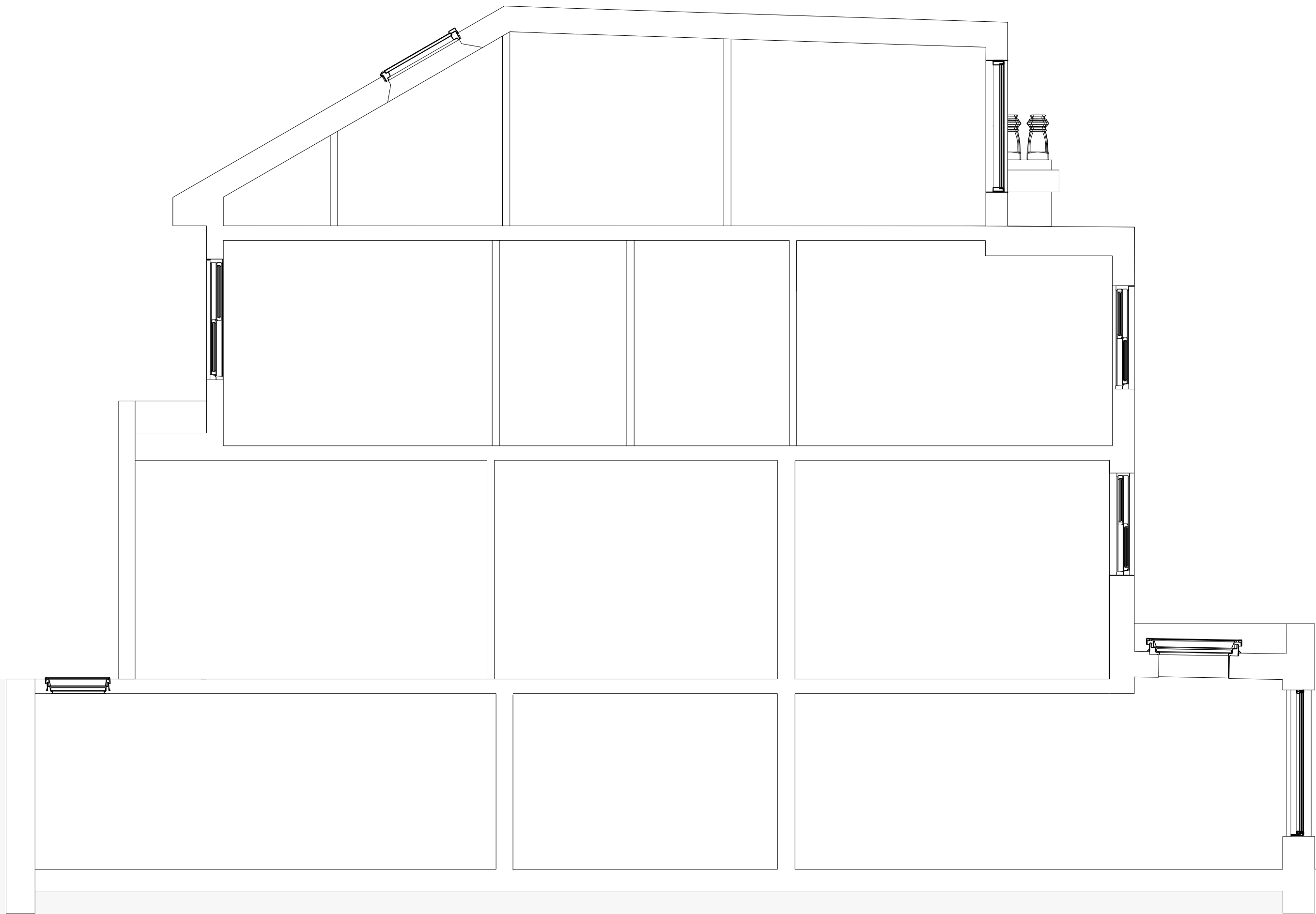
2 Proposed Section 1 : 50
