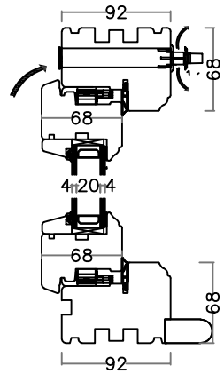
Vertical Section
