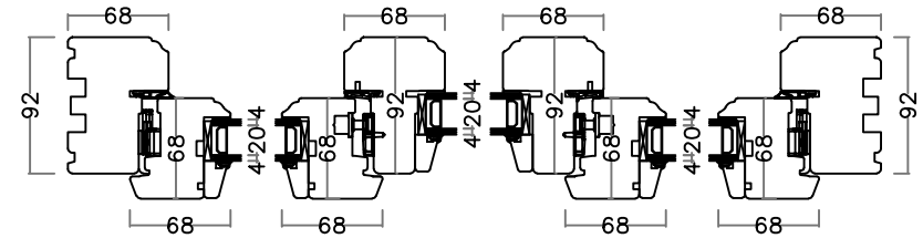
Horizontal Detail
