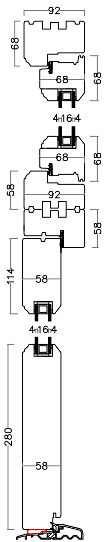
Vertical Section
