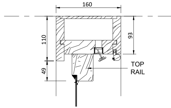
DETAIL A - TYPICAL HEAD SECTION @ 1:5
