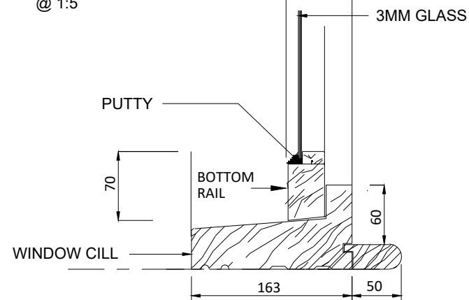
DETAIL C - TYPICAL CILL SECTION @ 1:5
