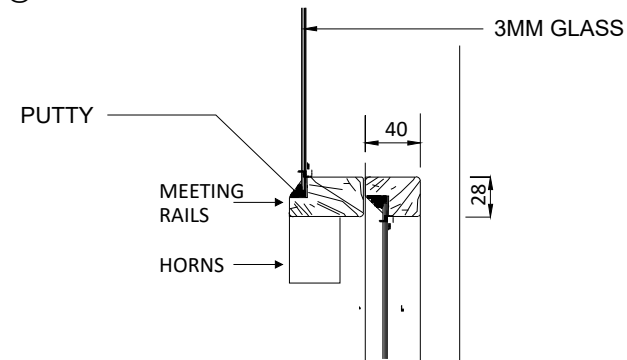
DETAIL B - TYPICAL CENTRE BAR SECTION @ 1:5
