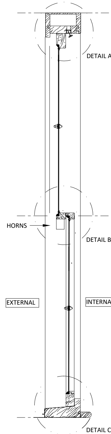
TYPICAL SECTION EXISTING TIMBER SINGLE GLAZED SASH WINDOW @ 1:10
