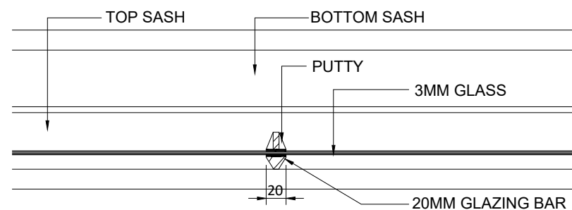
DETAIL D - TYPICAL GLAZING BAR SECTION EXISTING TIMBER SINGLE GLAZED SASH WINDOW @ 1:5
