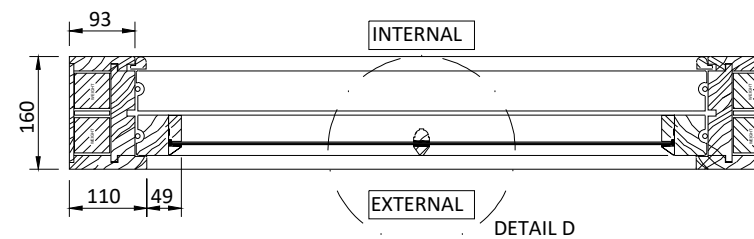
WINDOW PLAN EXISTING TIMBER SINGLE GLAZED SASH WINDOW @ 1:10
