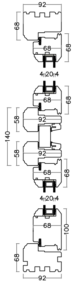
Vertical Section
