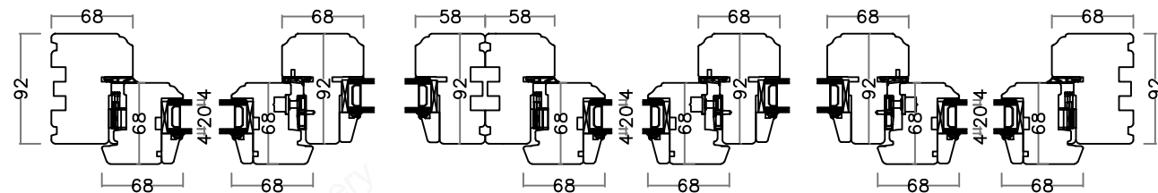
Horizontal Detail
