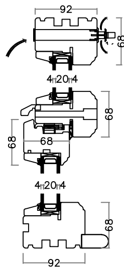
Vertical Section
