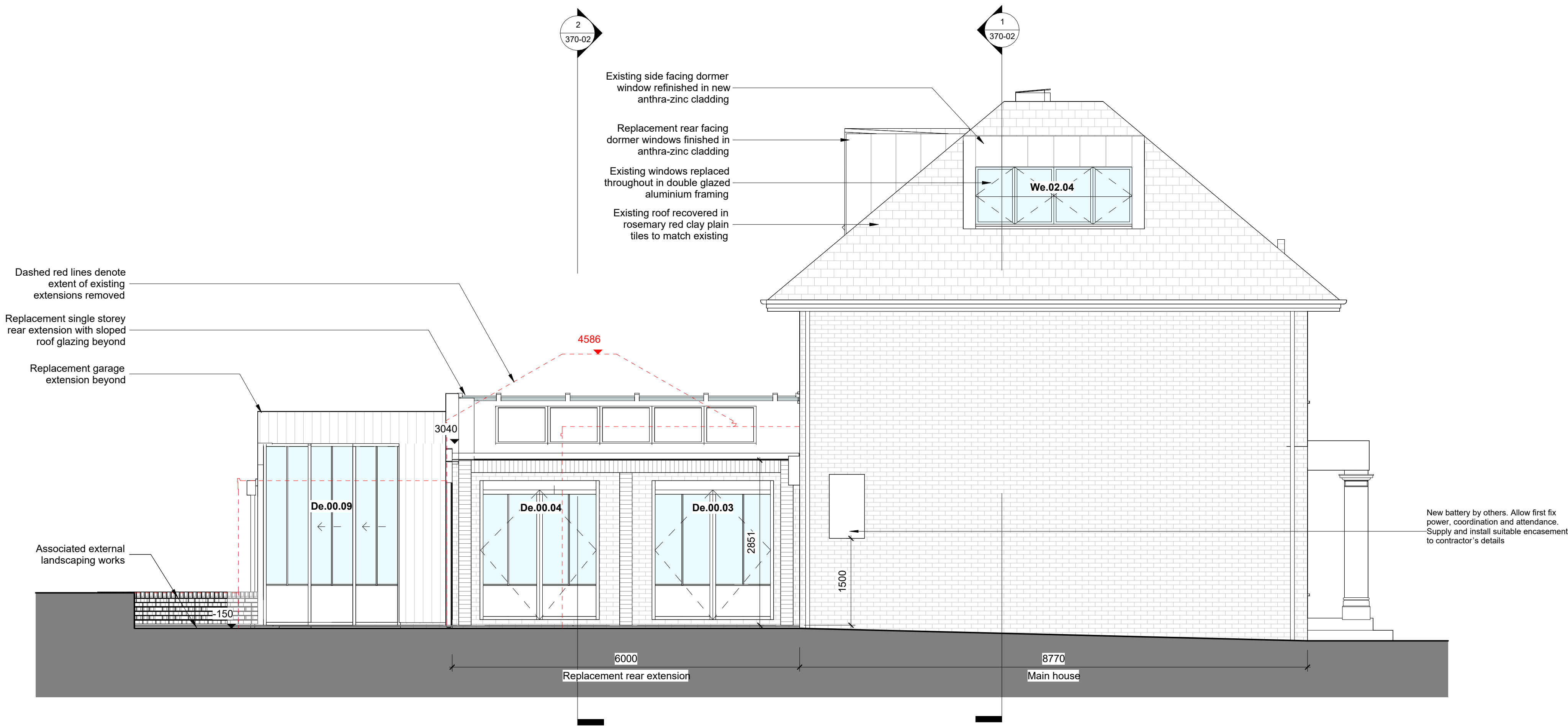
1 Proposed Side Elevation 1 1 : 50
