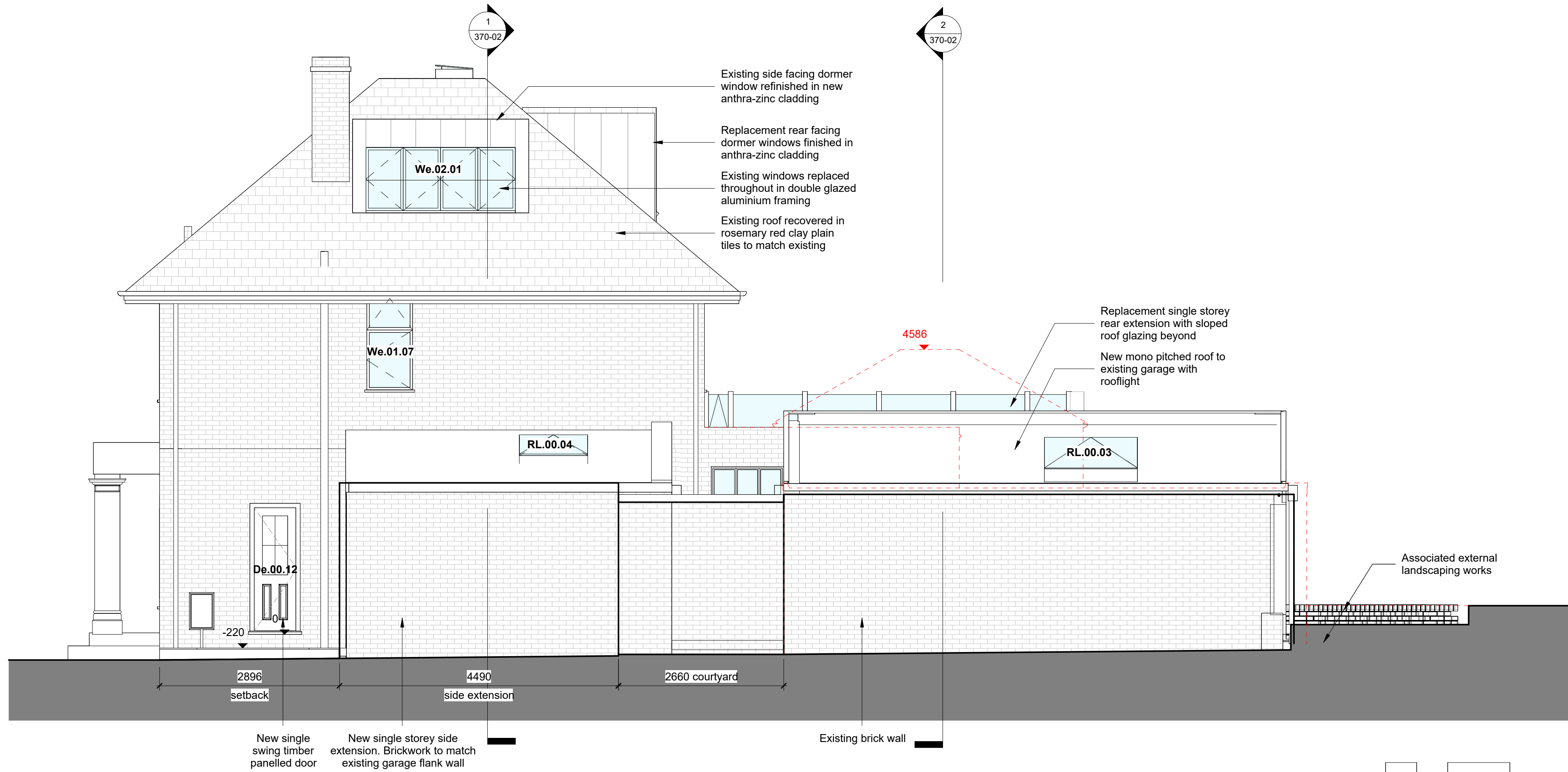
2 Proposed Side Elevation 2 1 : 50
