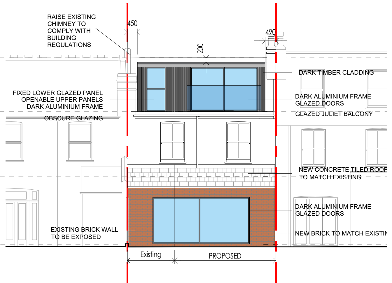
REAR ELEVATION as proposed 1:100
