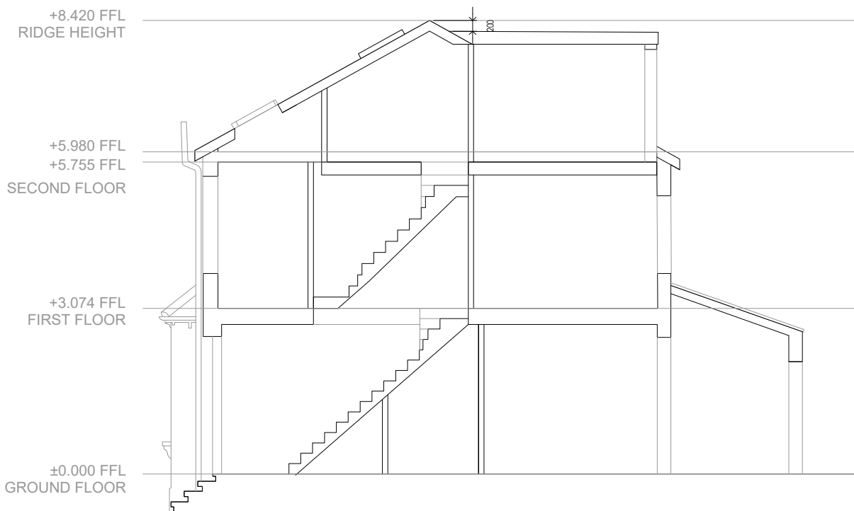
TYPICAL SECTION as proposed 1:100
