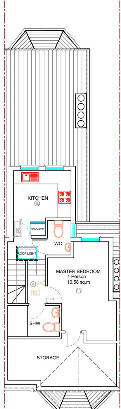
EXISTING LOFT PLAN 1:100
