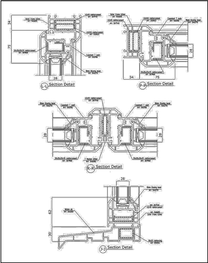
2 Proposed Typical uPVC Casement Window Section Details - W08 to W14 Scale: 1:5 @ A3
