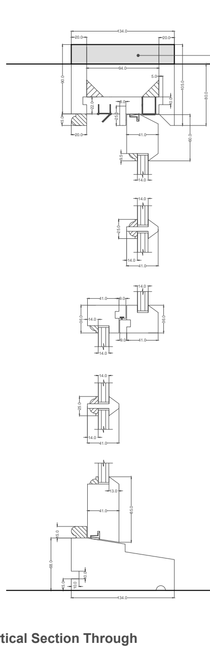
1 Proposed Typical Timber Sliding Sash Window Section Details - W01 & W02 Scale: 1:5 @ A3
