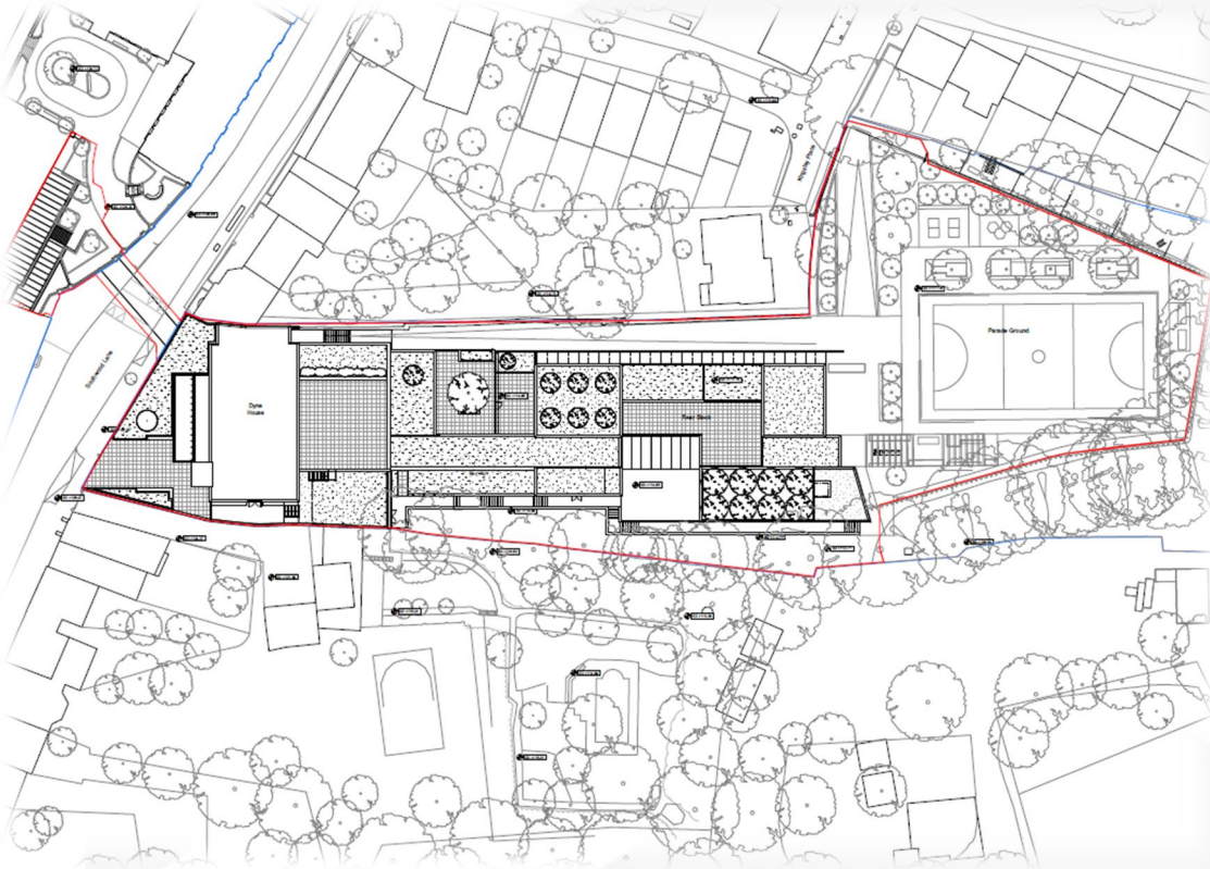
Figure 4: Proposed Site Plan, Drawing No. A/HS-DH3_2400_Rev.D (Hopkins Architects Limited)
