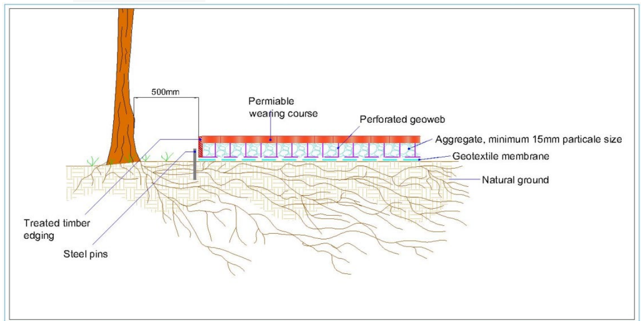
Figure 8: Typical cross-section for multi-dimensional confinement system using timber edging
