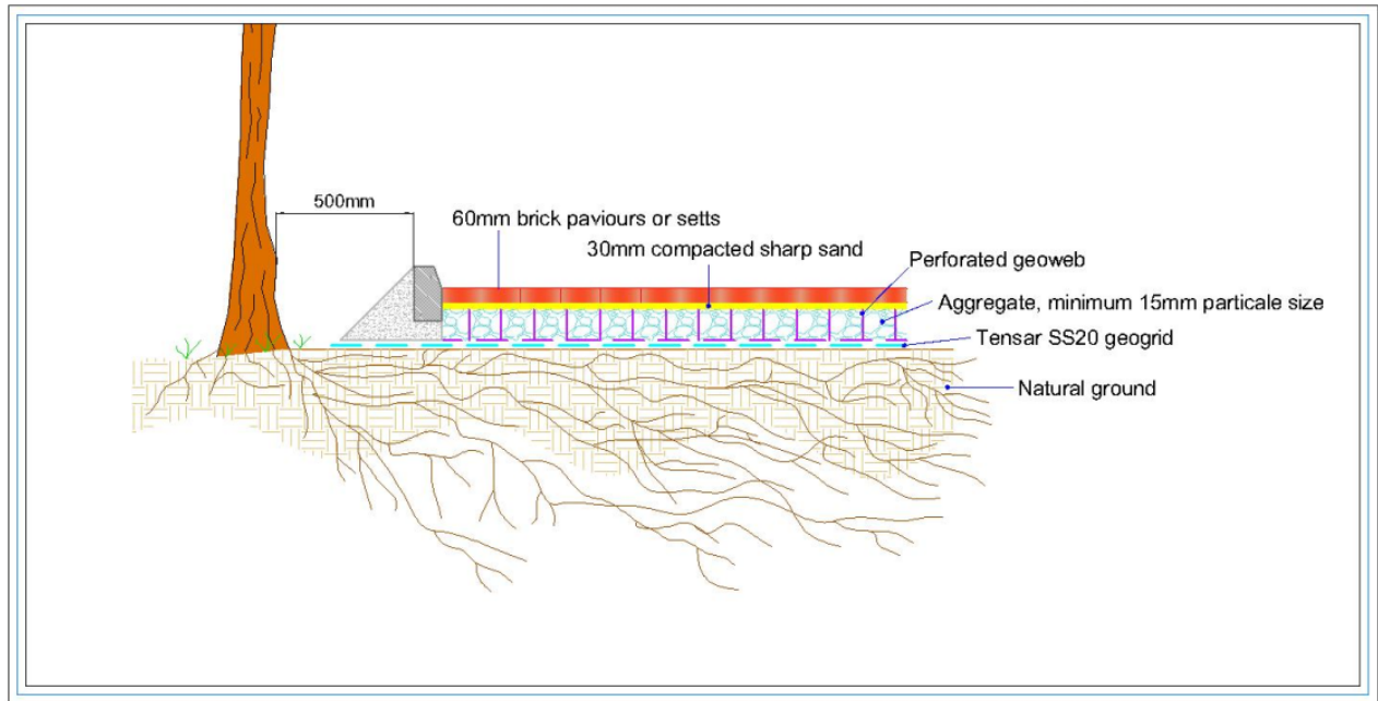
Figure 7: Typical cross-section for multi-dimensional confinement system using kerb edging
