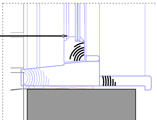
B 1:5 Typical replacement window detail
