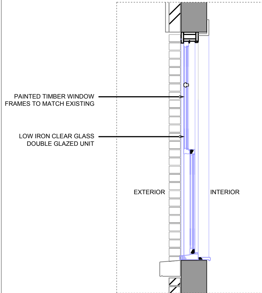
A 1:20 Typical replacement window detail
