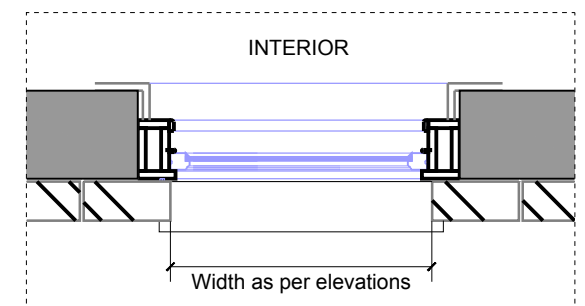
F 1:20 Section C-C
