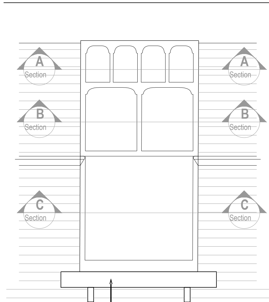
C Elevation
