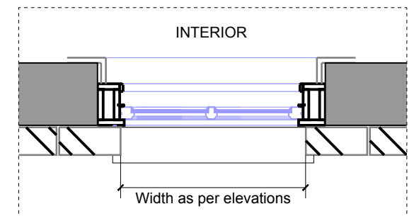
E 1:20 Section B-B
