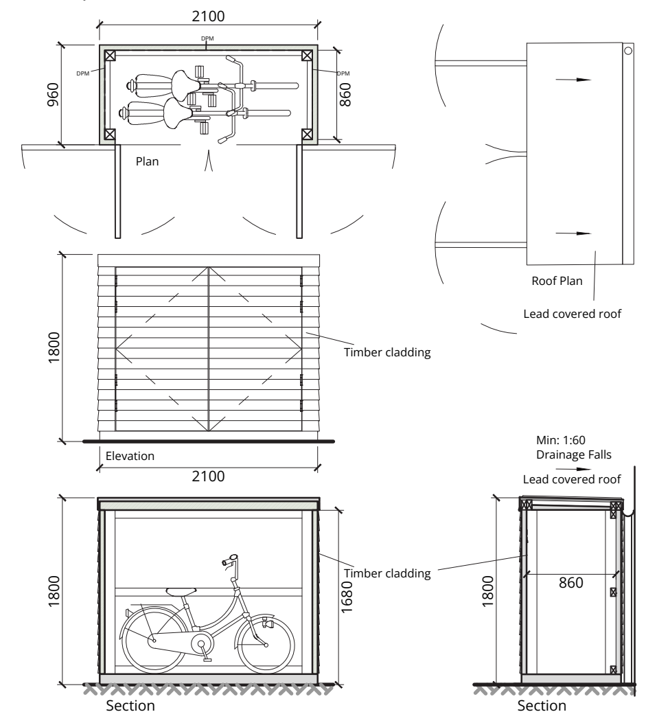
Bike Storage 1:50
