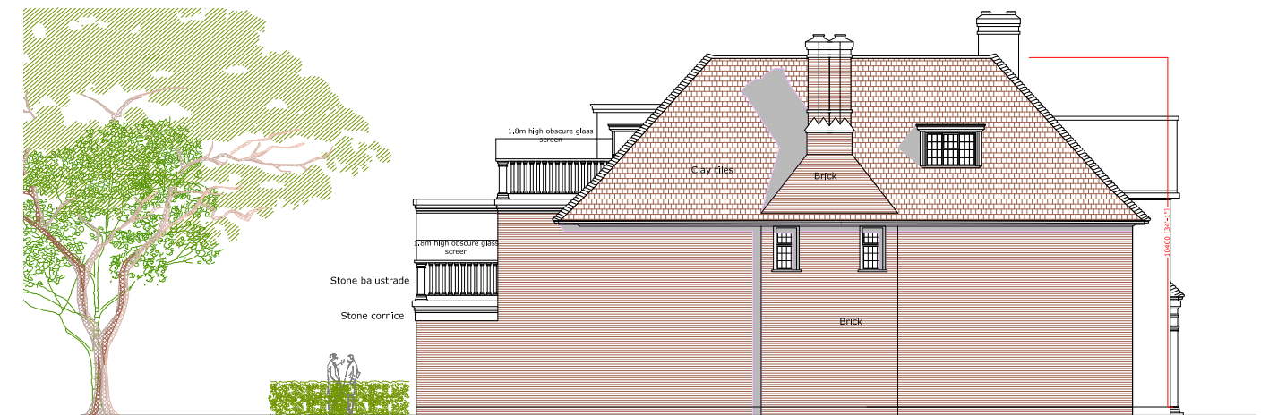
2017 ref: HGY/2016/3876 Proposed Side Elevation
