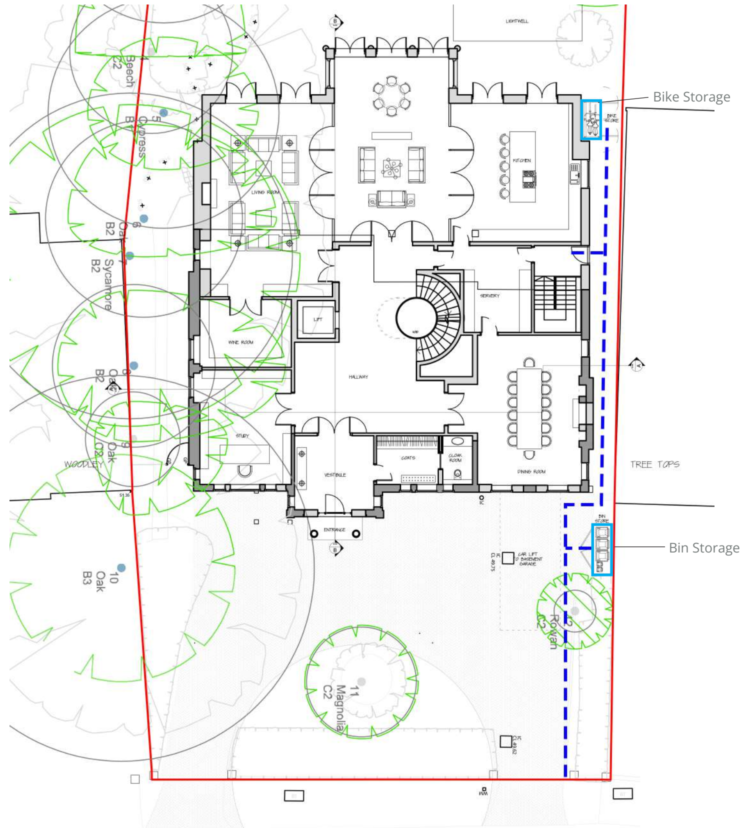
Bike and Bin Storage Site Plan 1:200
