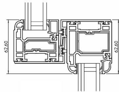
Meeting Rail
