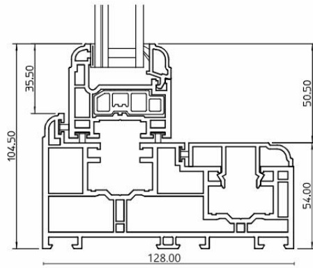
Top Rail
