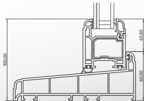
Bottom Rail
