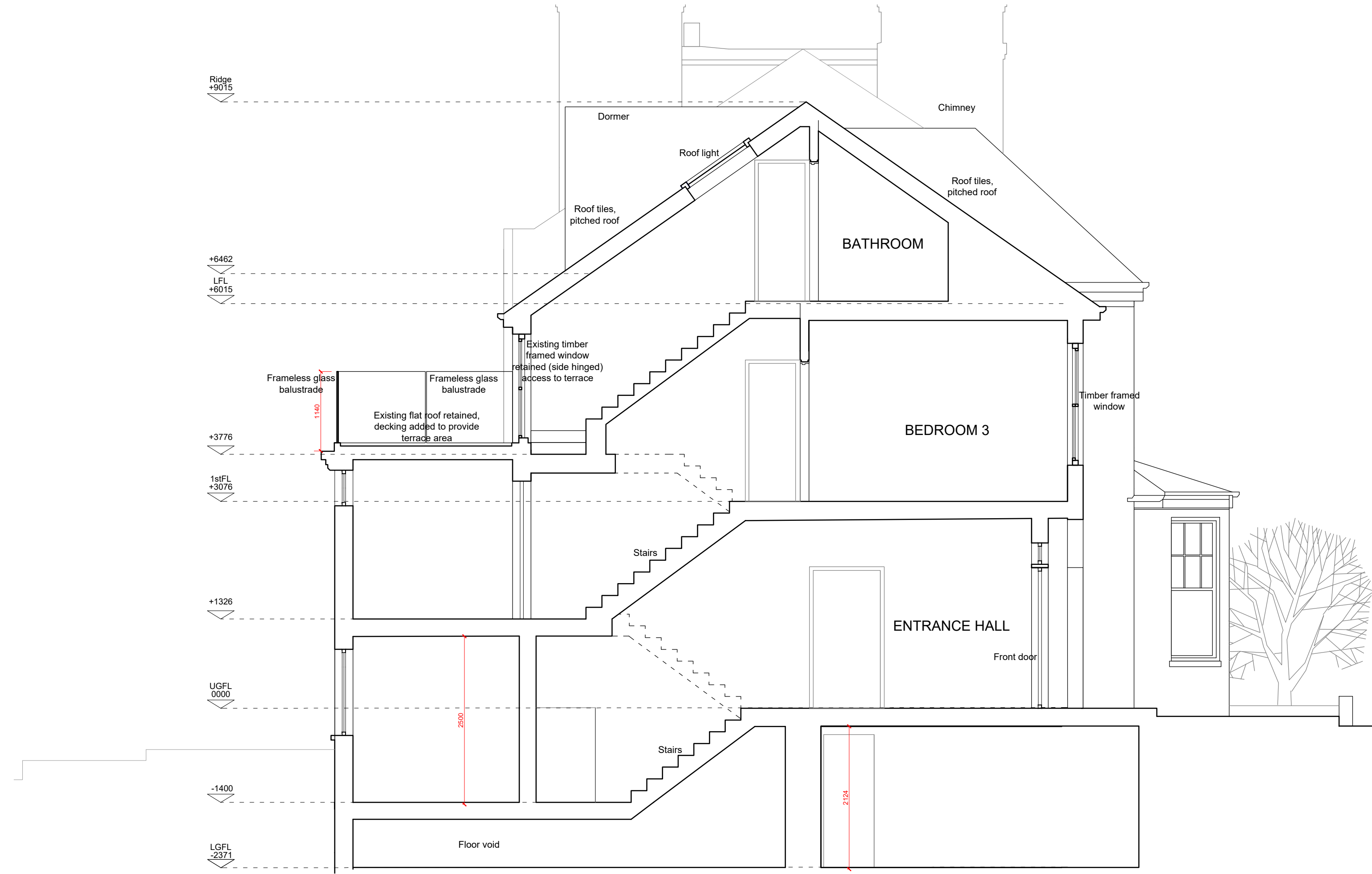
Existing Section B-B
