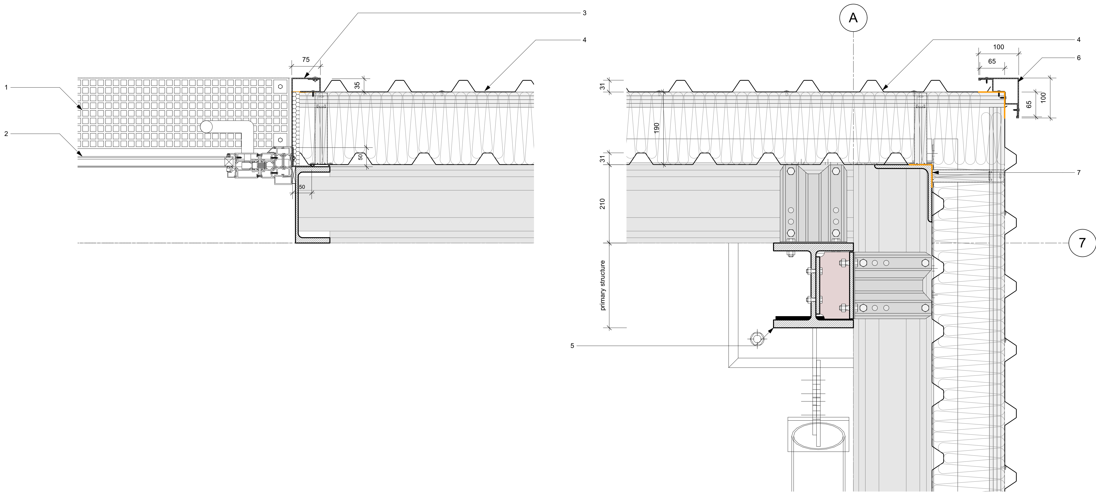
2 Typical Corrugate to Corrugate Corner Junction Scale: 1:5
