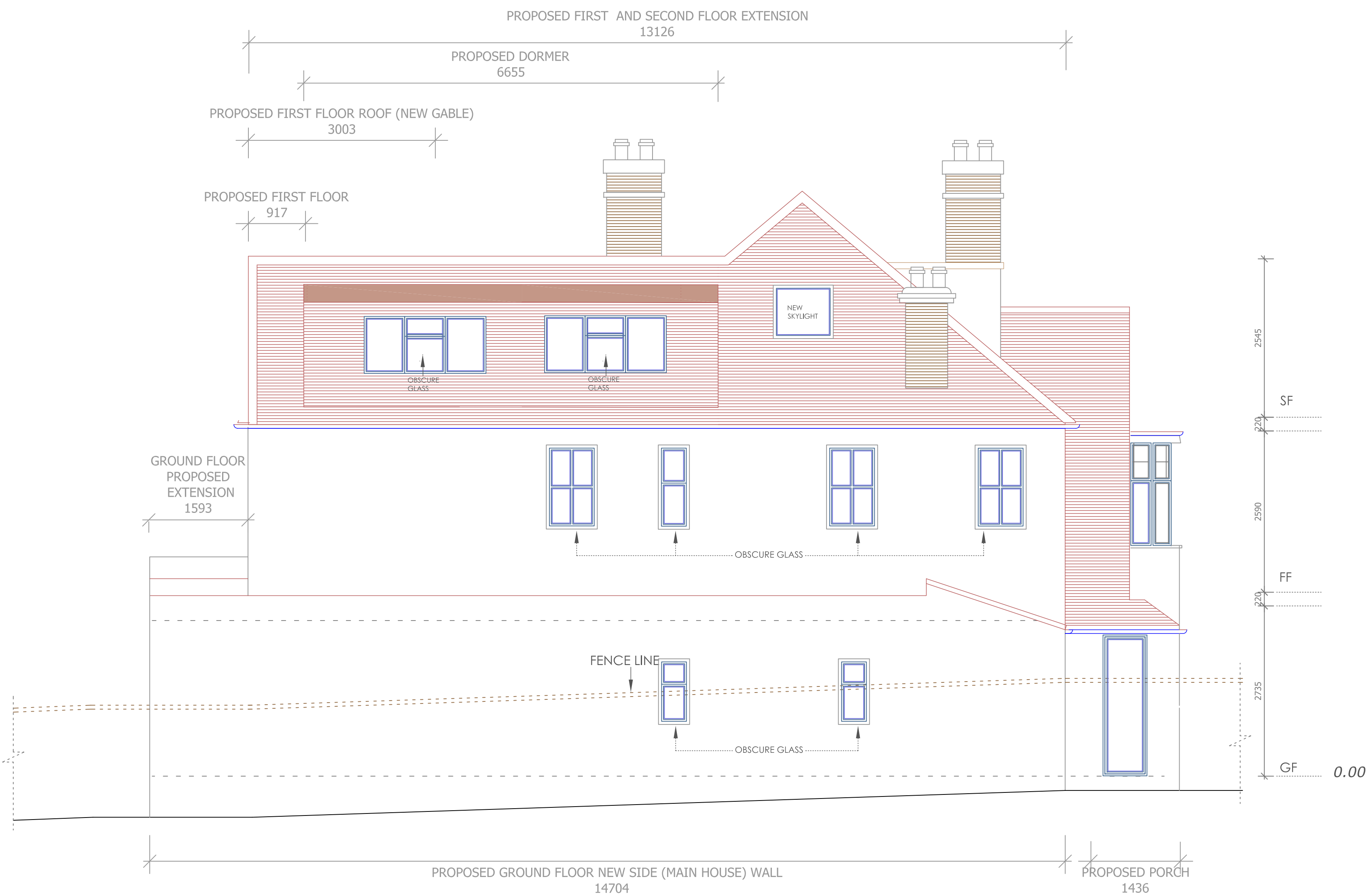
ELE PROPOSED SIDE EAST ELEVATION
