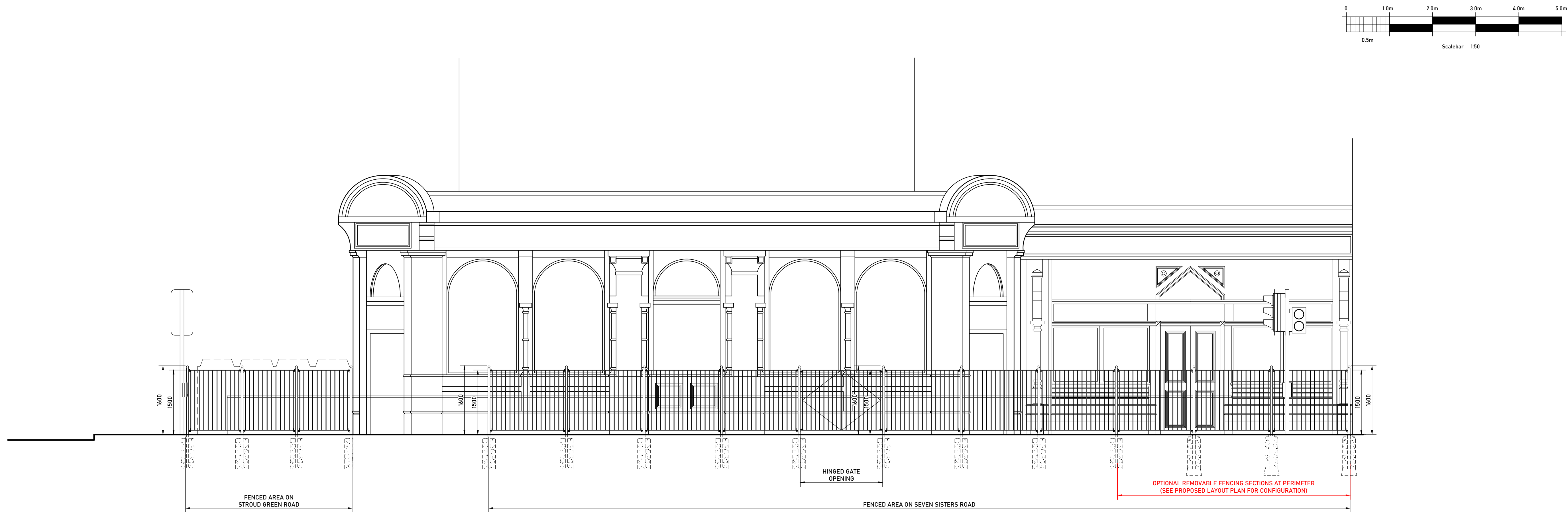
ELEVATION 1-1. SEVEN SISTERS ROAD ELEVATION.
