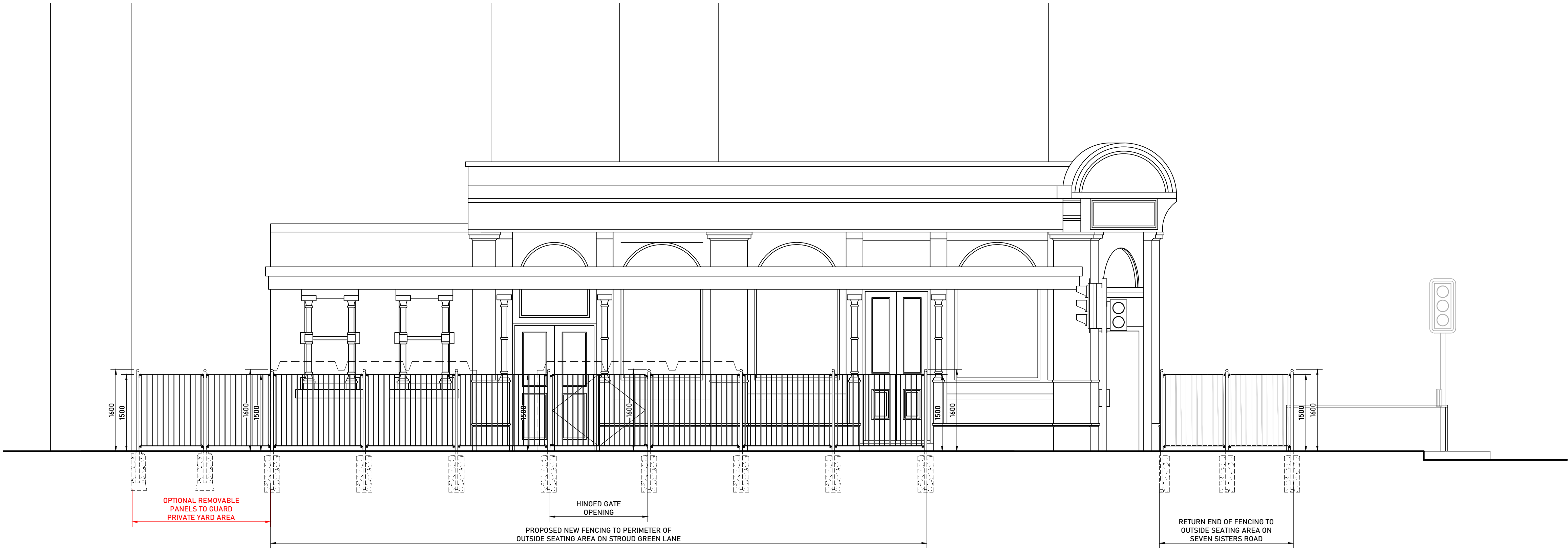
ELEVATION 2-2. STROUD GREEN ROAD ELEVATION.
