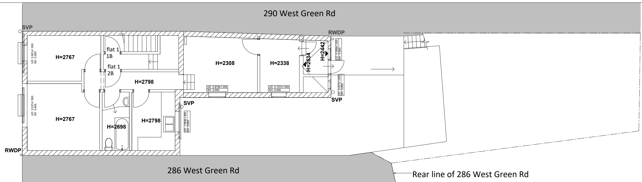
existing first floor ga plan
