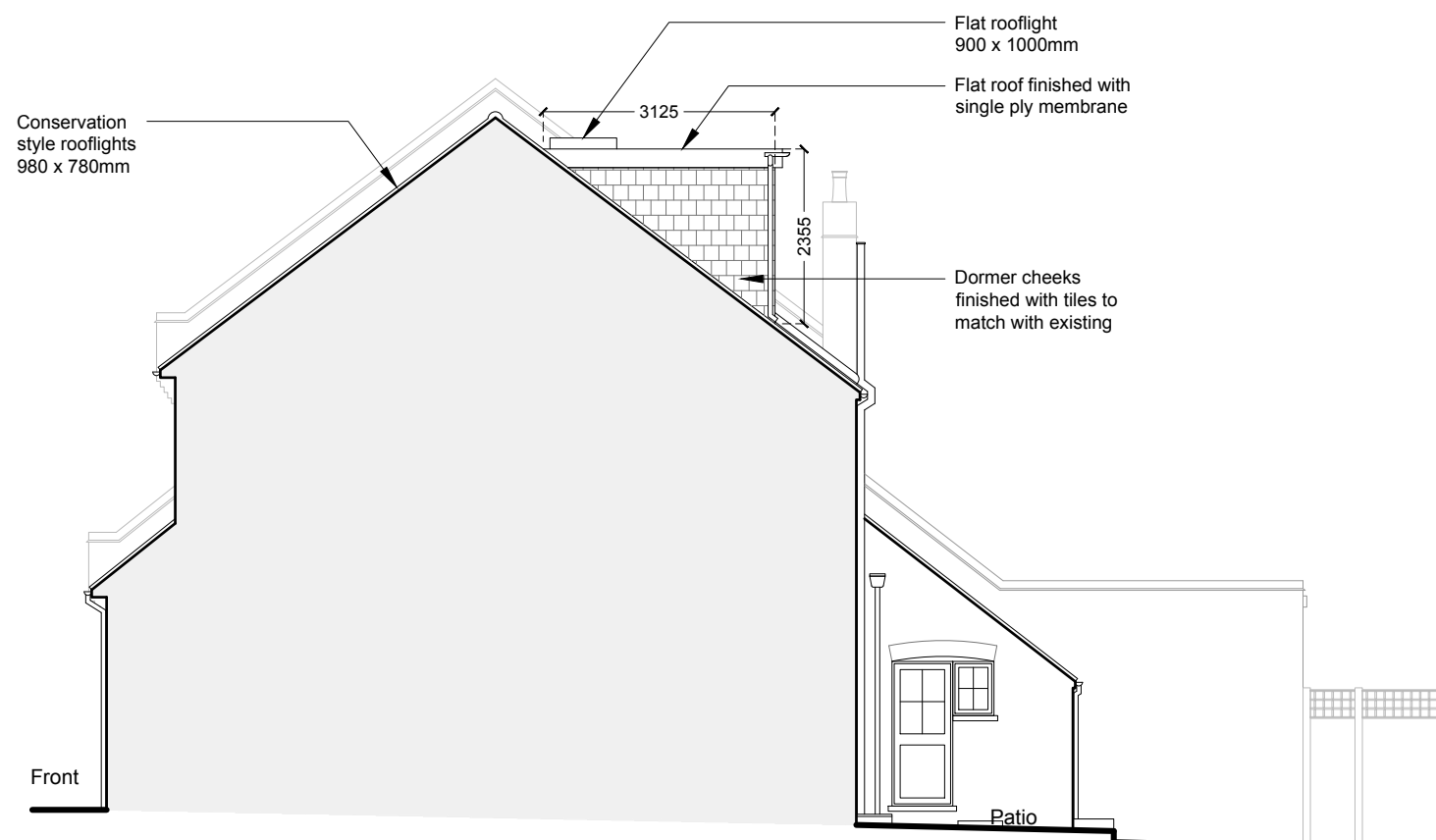
Side Elevation As Proposed 1:100
