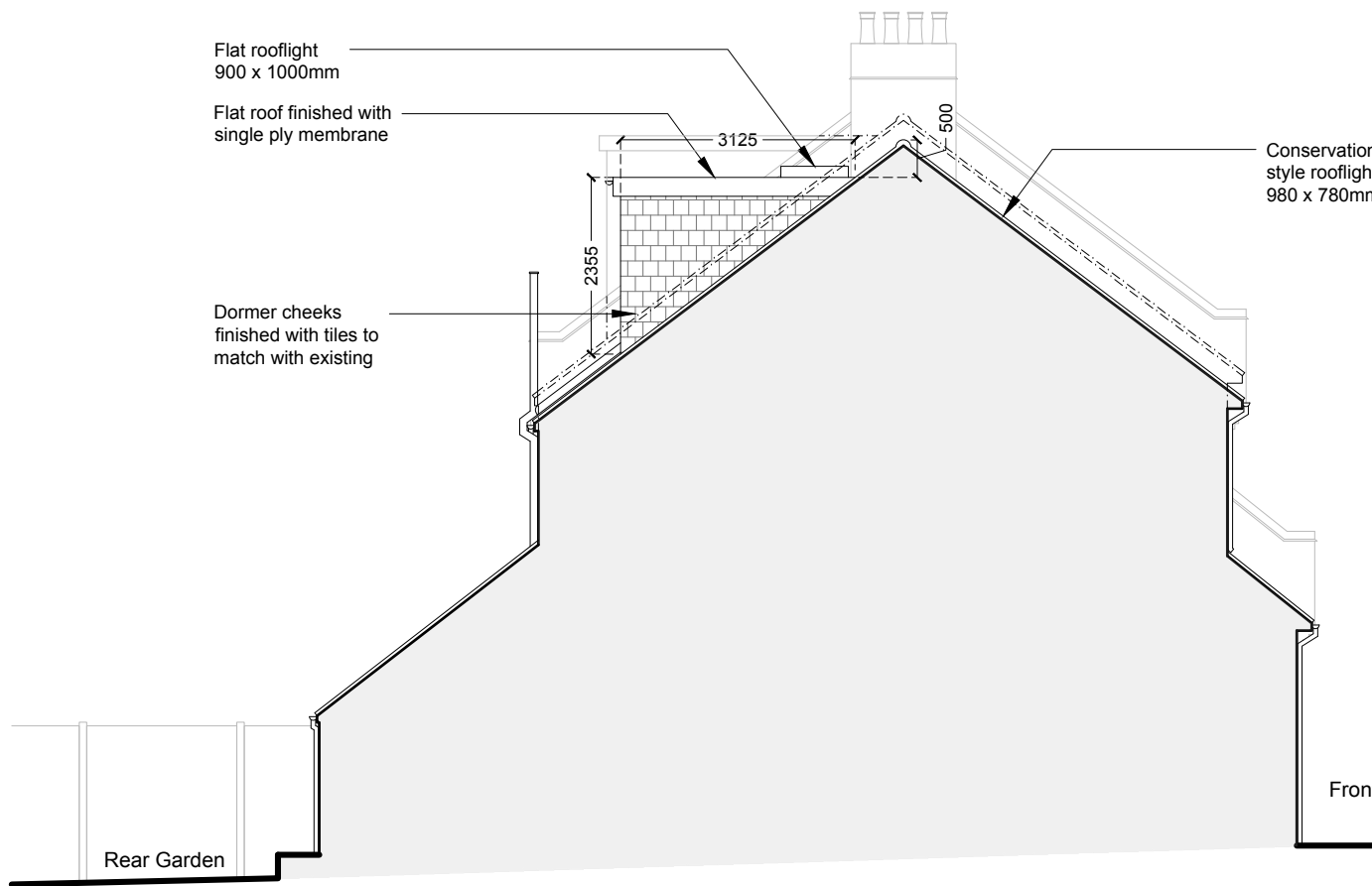
Side Elevation As Proposed 1:100
