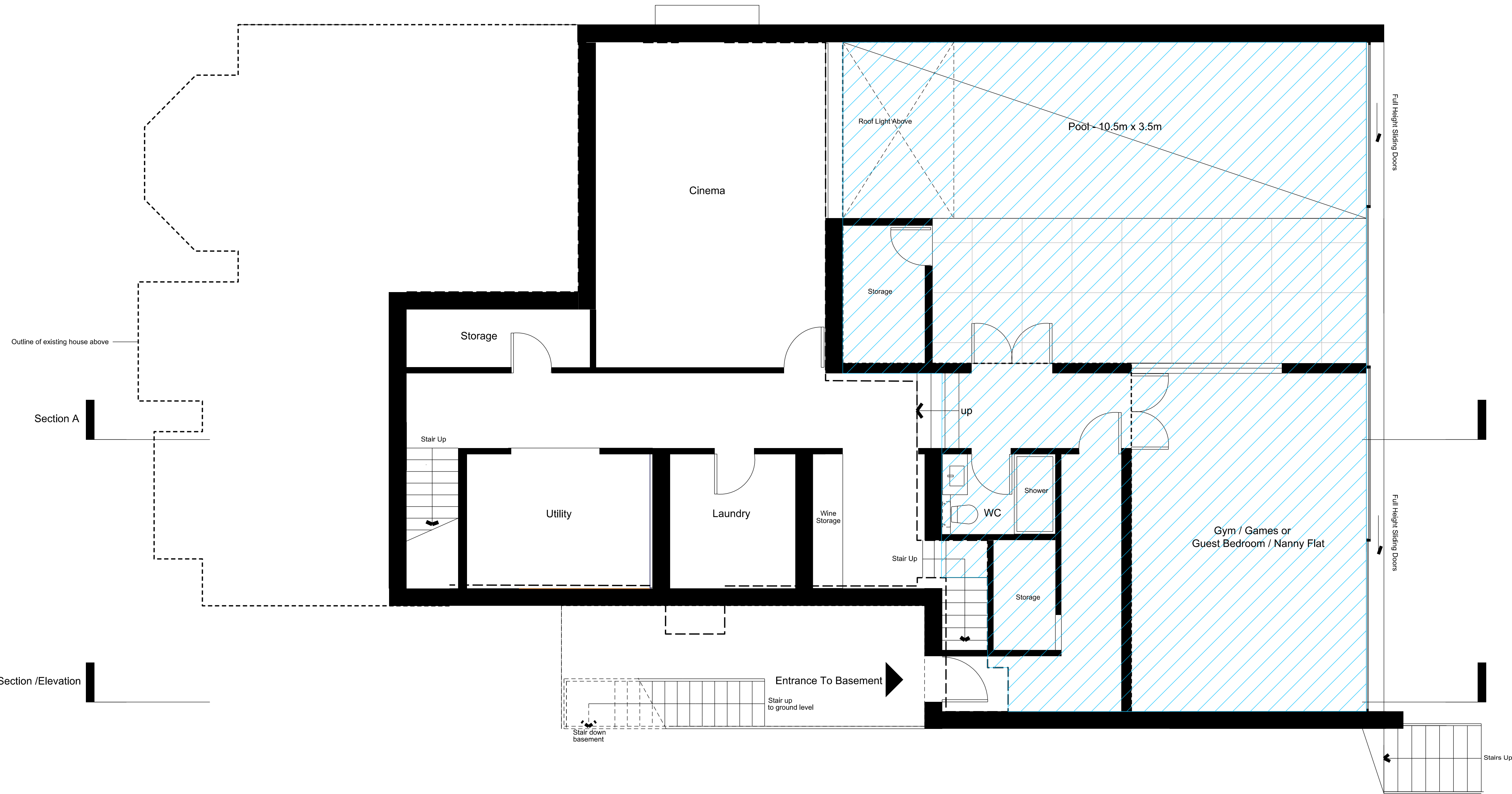
PROPOSED BASEMENT PLAN 210m2 GIA
