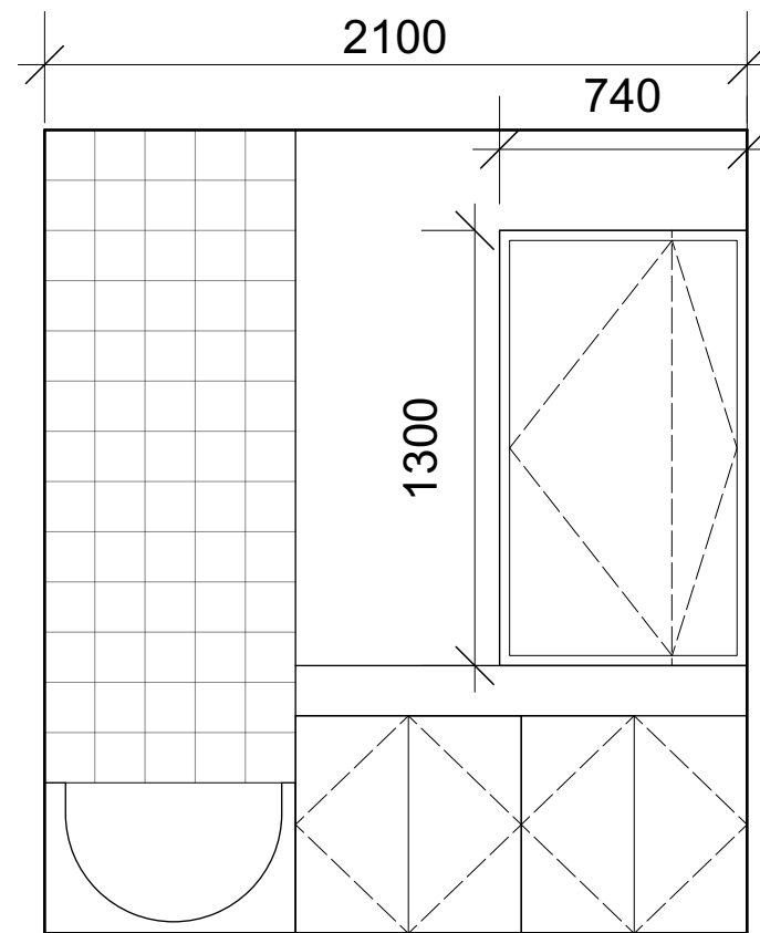
ELEVATION C
