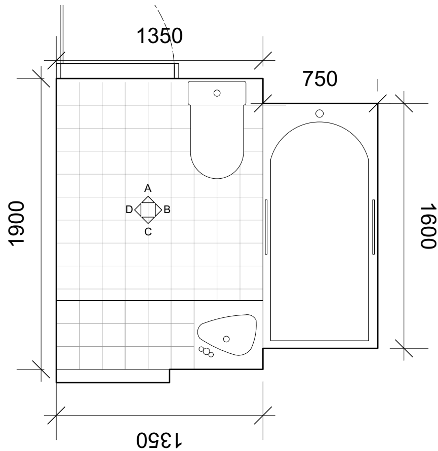
FLOOR PLAN
