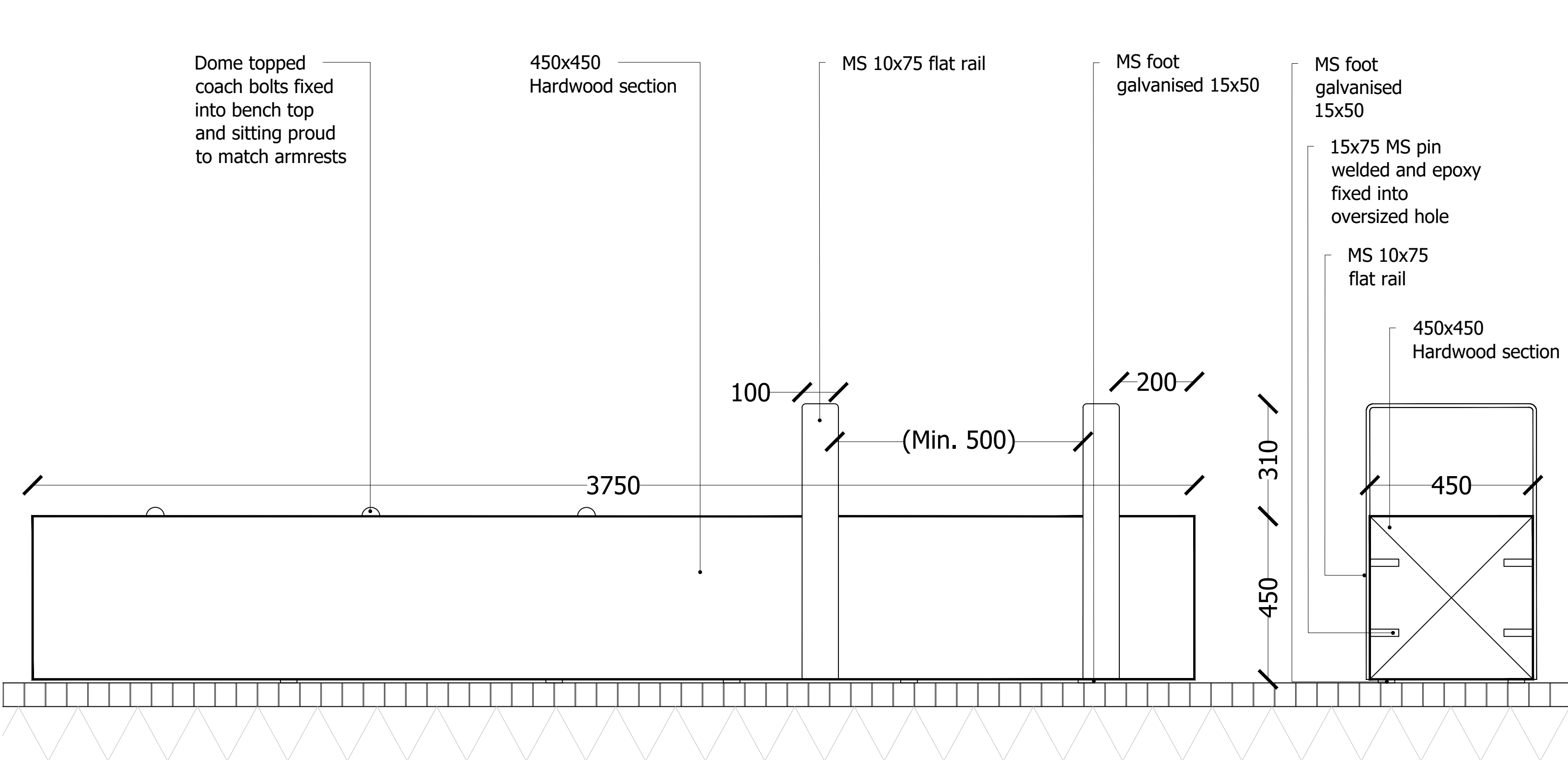
01 BS1 - SOLID TIMBER BENCH WITH ARMRESTS 1:10@A0
