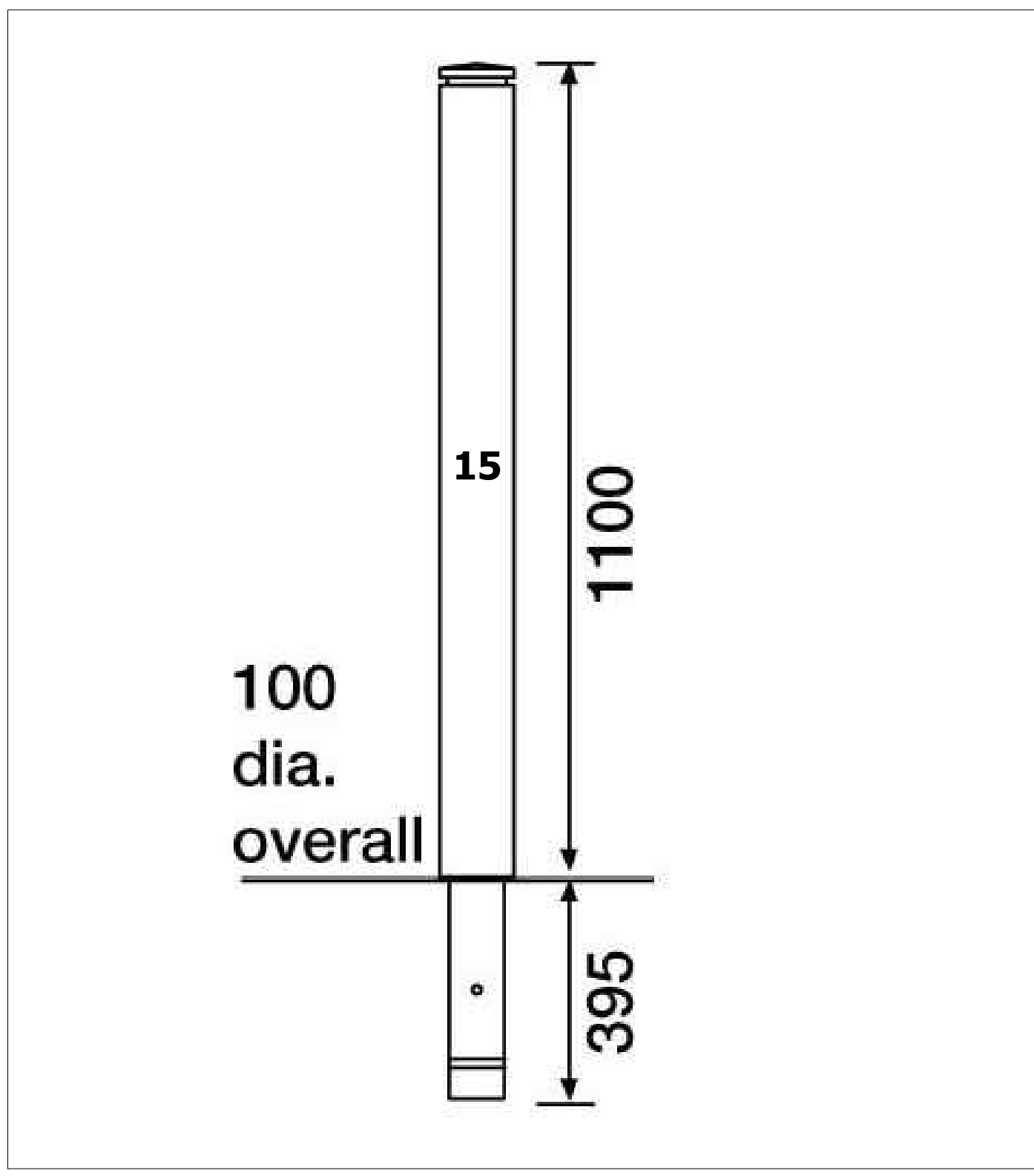
02 BL1 - STEEL BOLLARD
