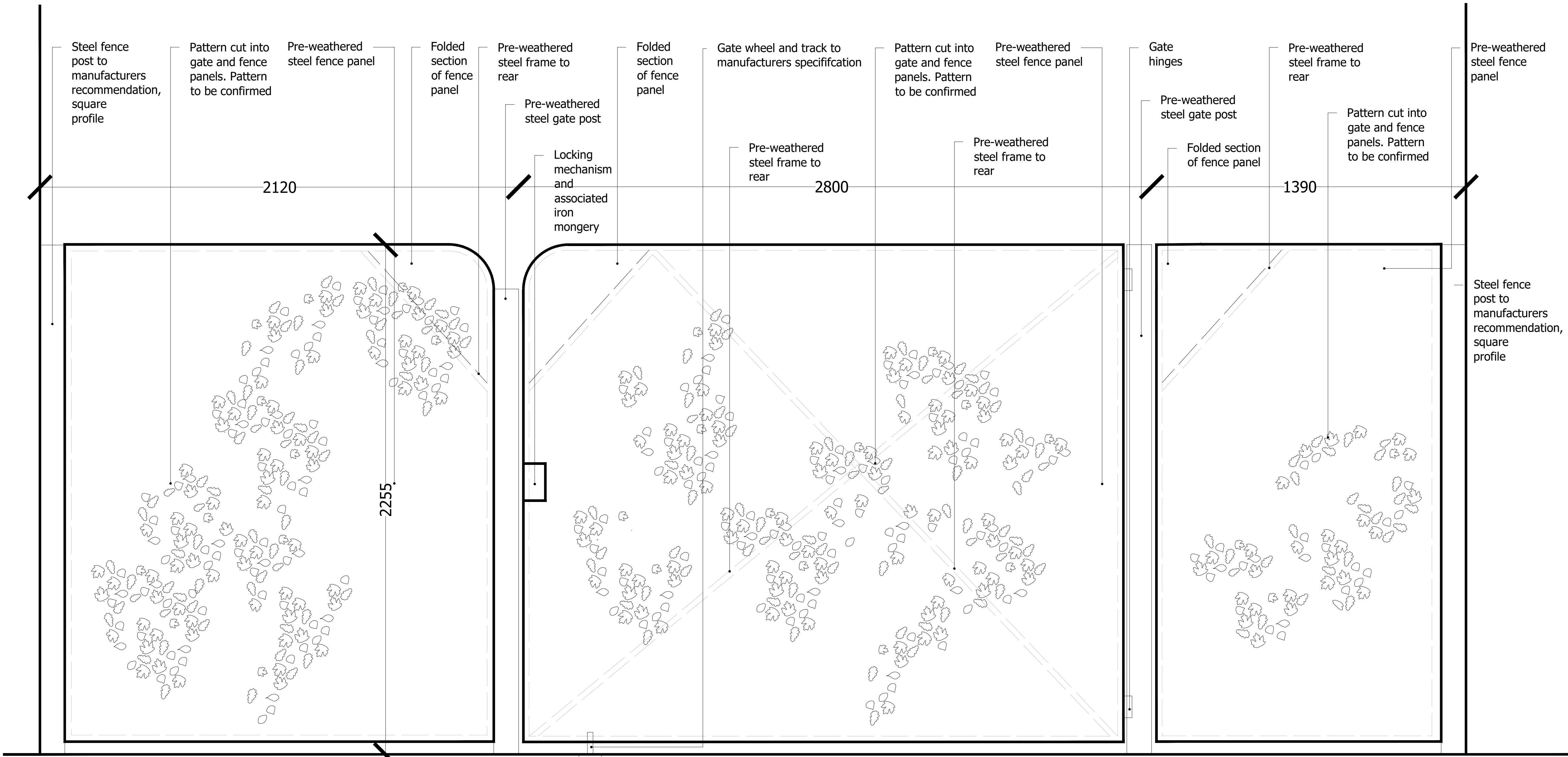
03 G2 - SINGLE LEAF GATE AND FENCING 1:10@A0
