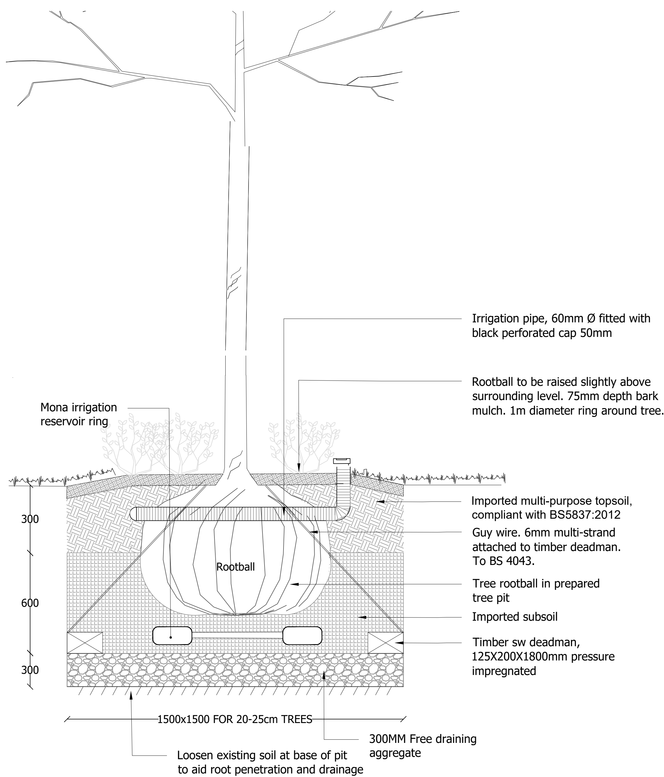
01 TREE PIT DETAIL/MULTISTEM PLANTER 1:10@A0
