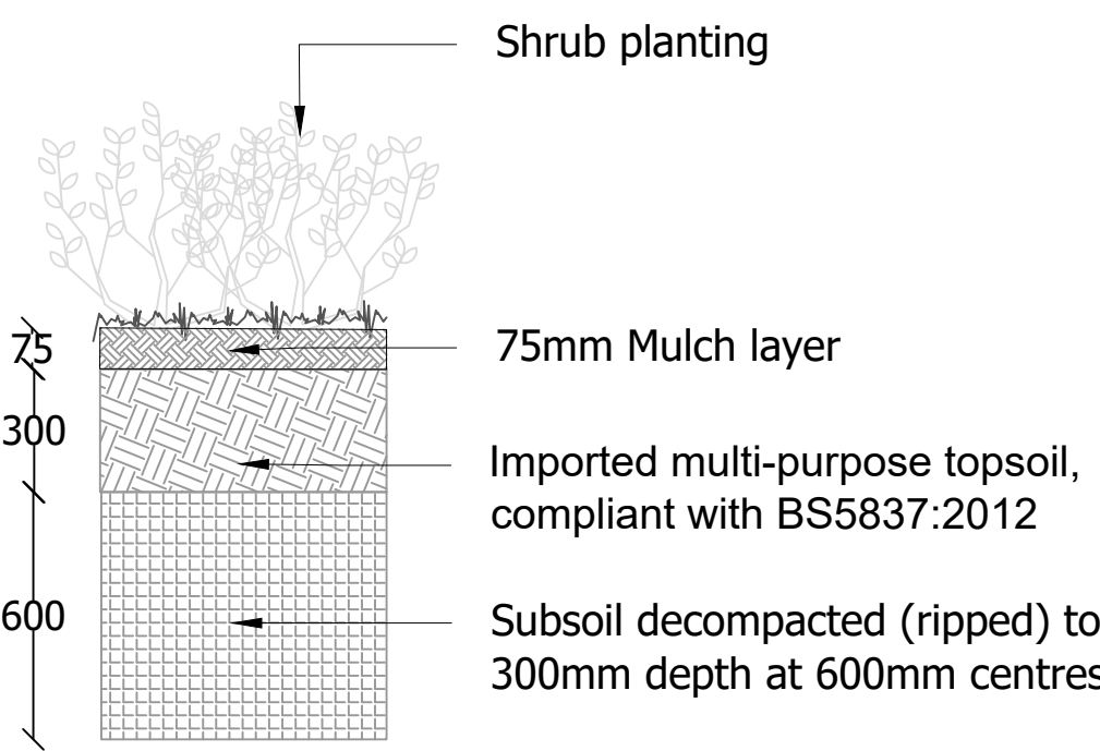
03 SHRUB DETAIL 1:10@A0
