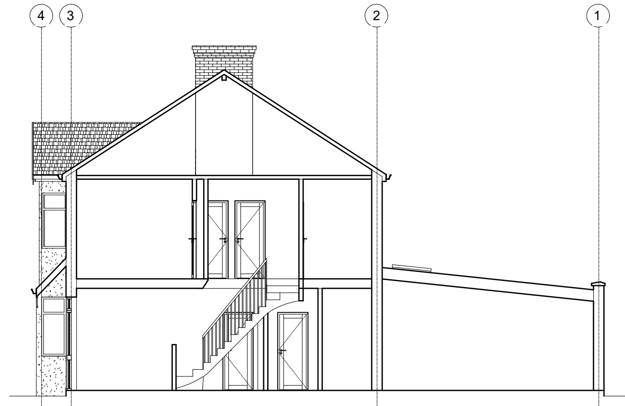
EXISTING SECTION
