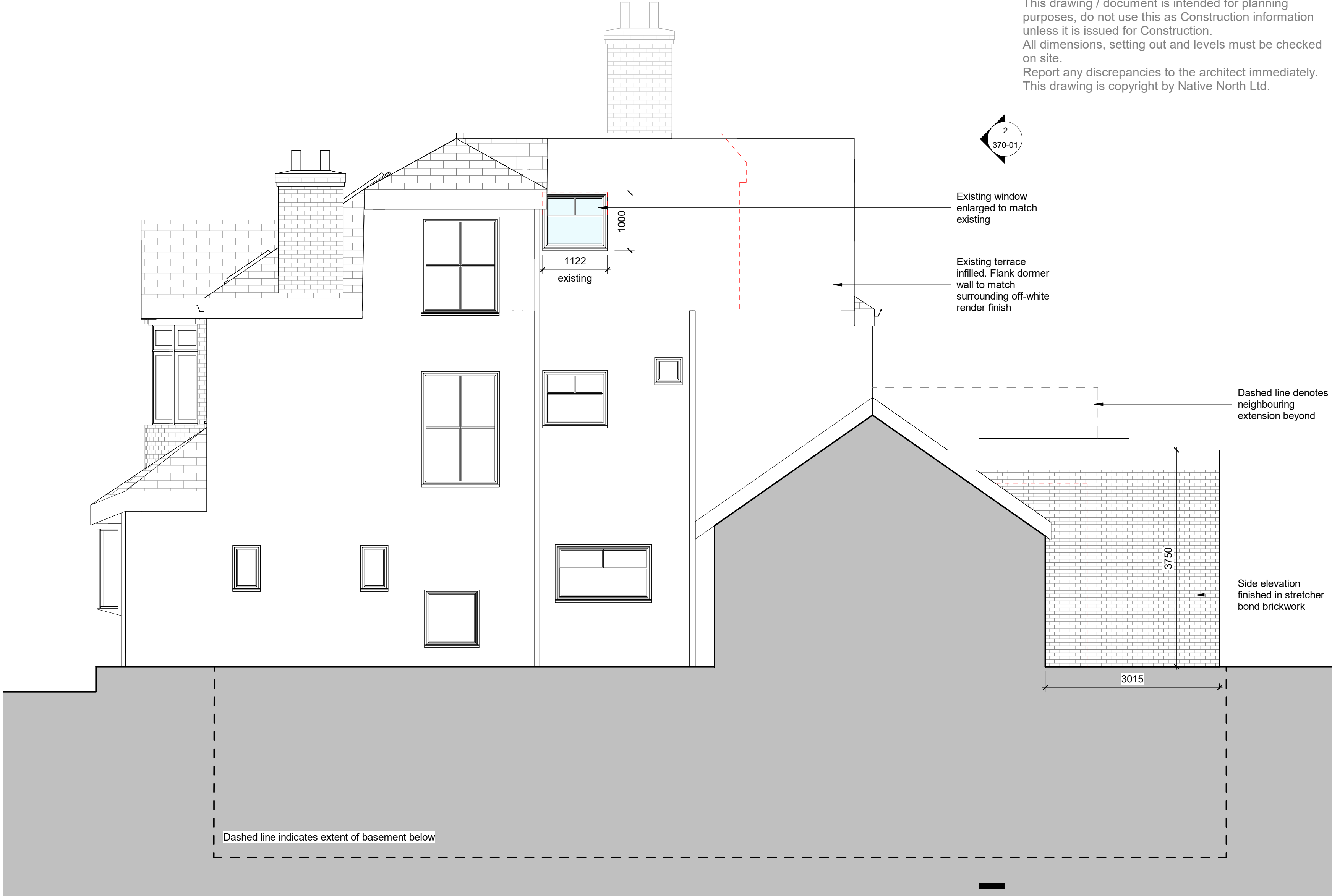
2 Proposed Side Elevation 1:50
