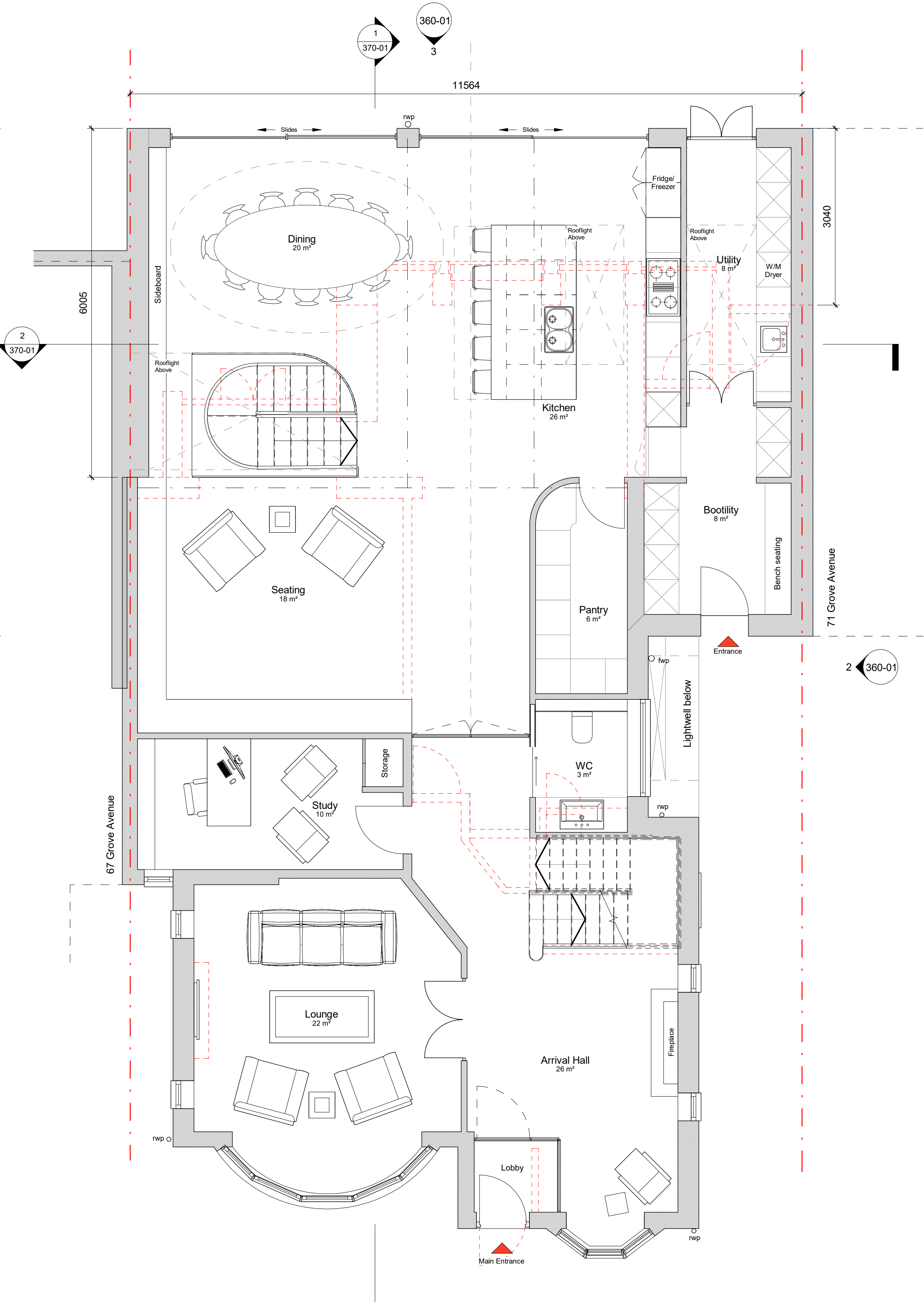
2 Proposed Ground Floor 1 : 50
