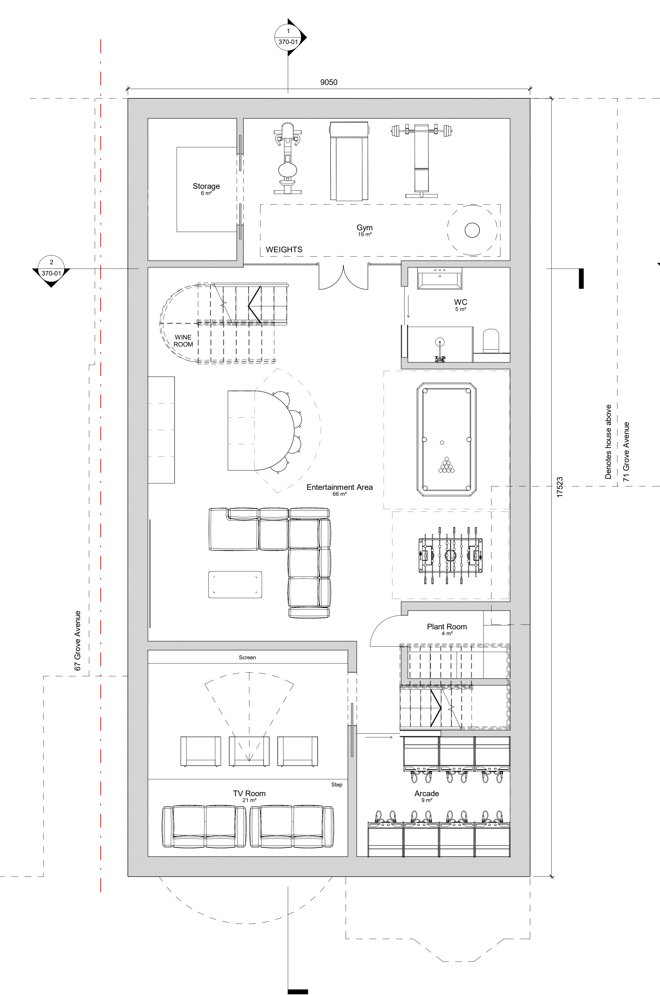
1 Proposed Basement 1 : 50
