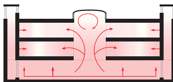
Figure 21: Passive Heating Strategy in Winter
