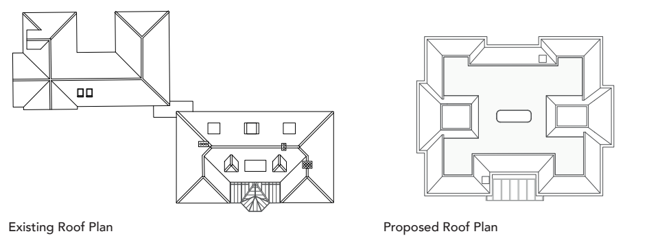
Figure 12. The roof plan of the existing Sproughton (Left) is 435 m 2 . The proposal merges the two volumes into a single building (Right) with a new footprint of 475 m 2 .
