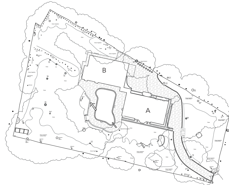
Figure 20. Existing Site Plan
