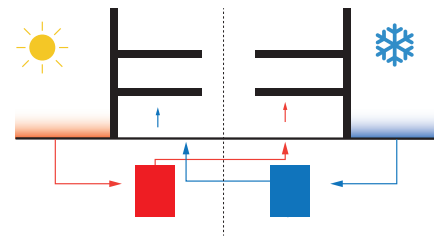
Figure 51: A thermal bank is essentially a temperature battery that stores cold and warm temperatures seasonally to supplement interseasonal heating and cooling demand.
