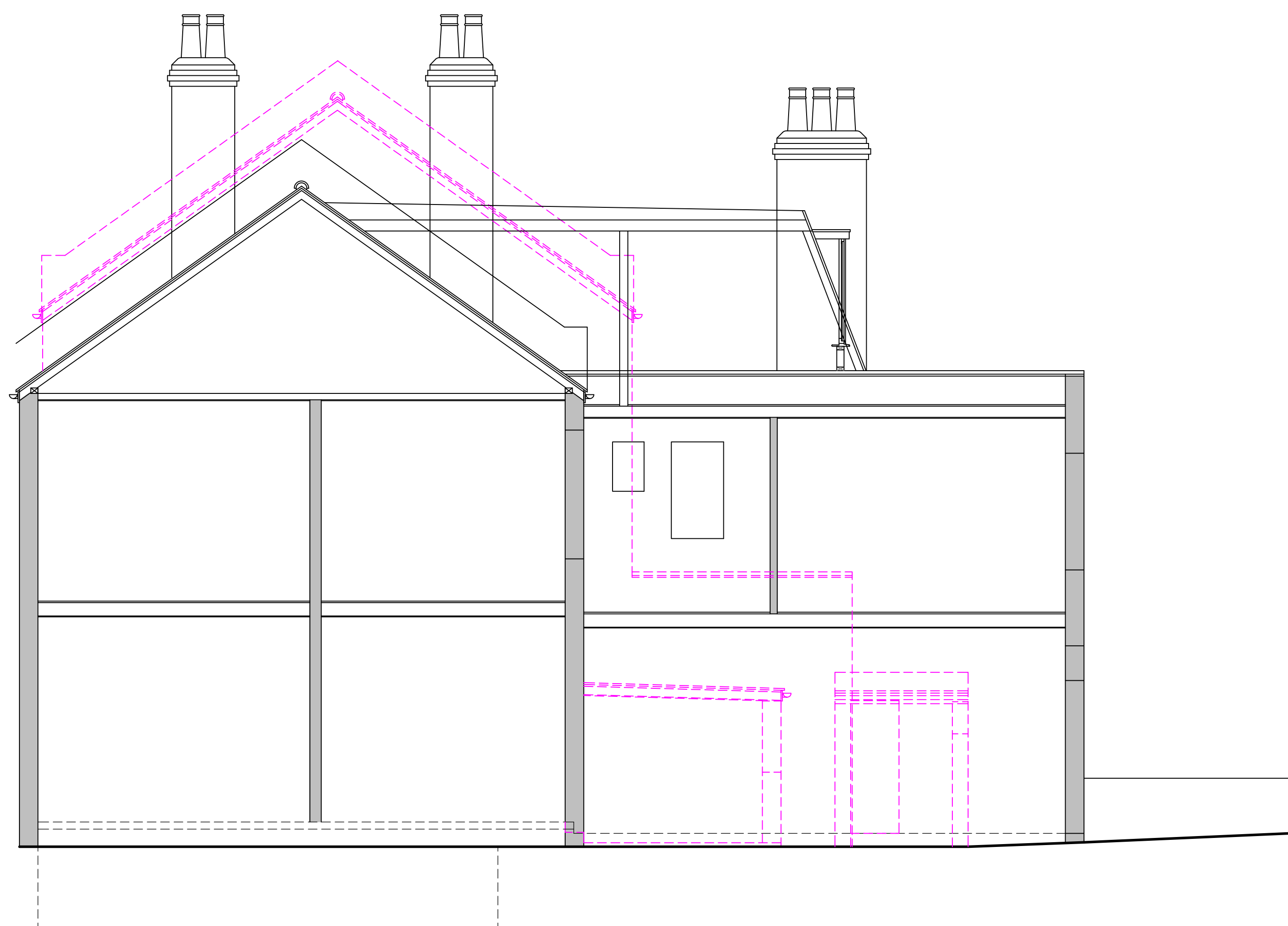
EXISTING SECTION 1:50
