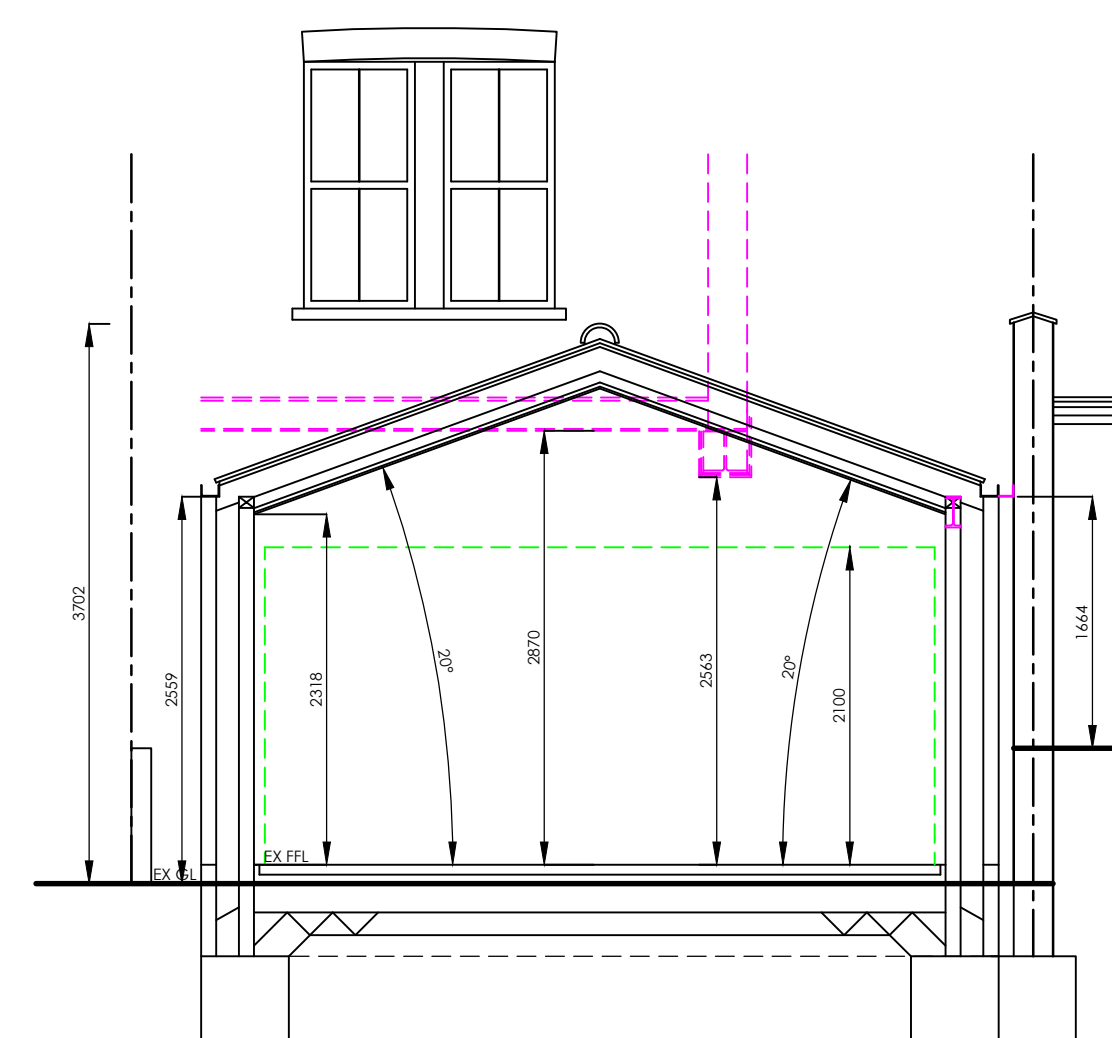
PROPOSED SECTION 1:50
