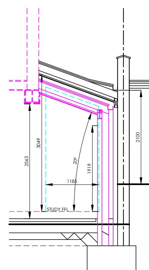
PROPOSED SECTION B - B 1:50
