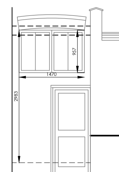
EXISTING ELEVATION WINDOW
