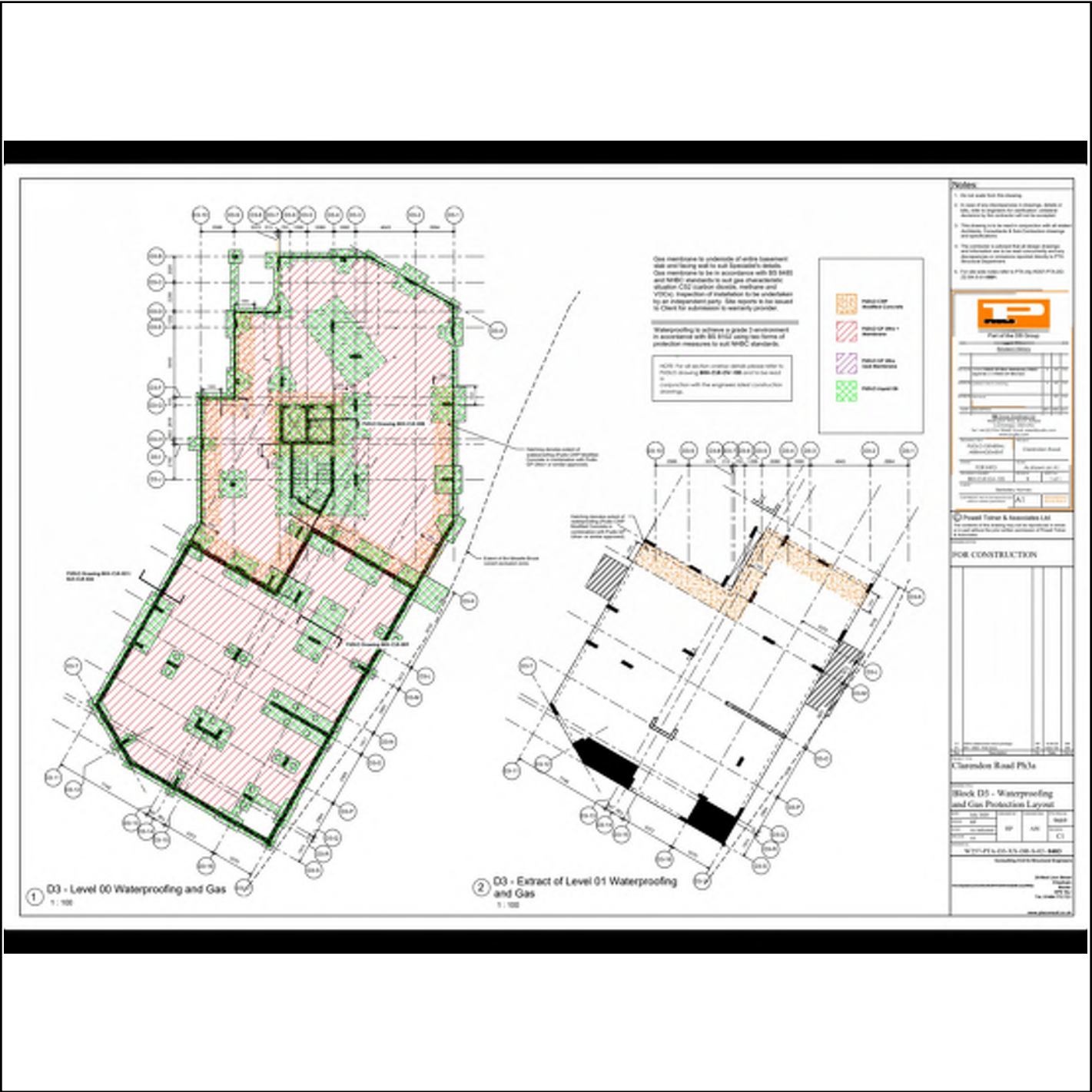
Block D3 Waterproofing and Gas Protection Layout
