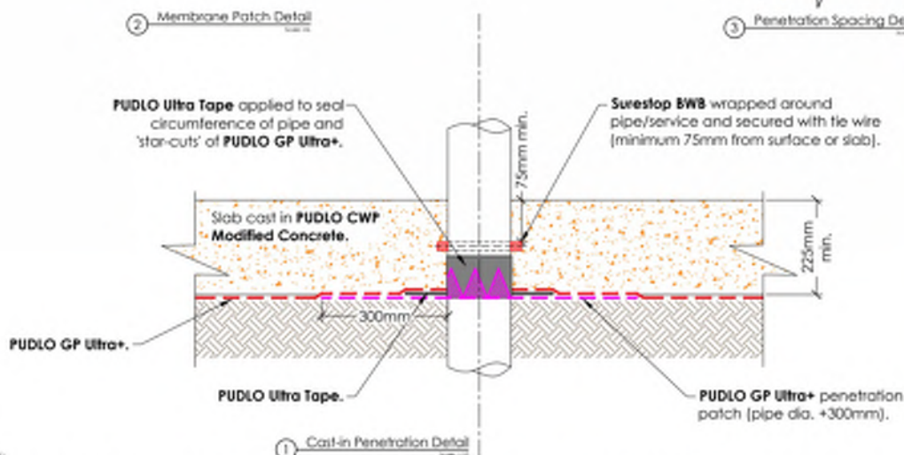
1 Cast-in Penetration Detail
