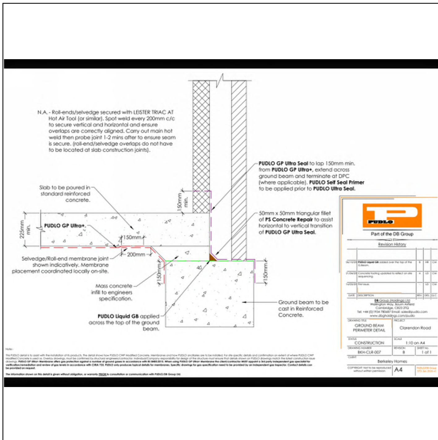
Ground Beam Perimeter Detail
