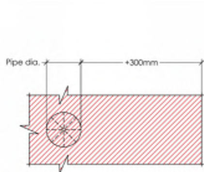
2 Membrane Patch Detail
