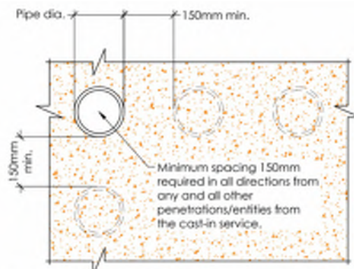
3 Penetration Spacing Detail
