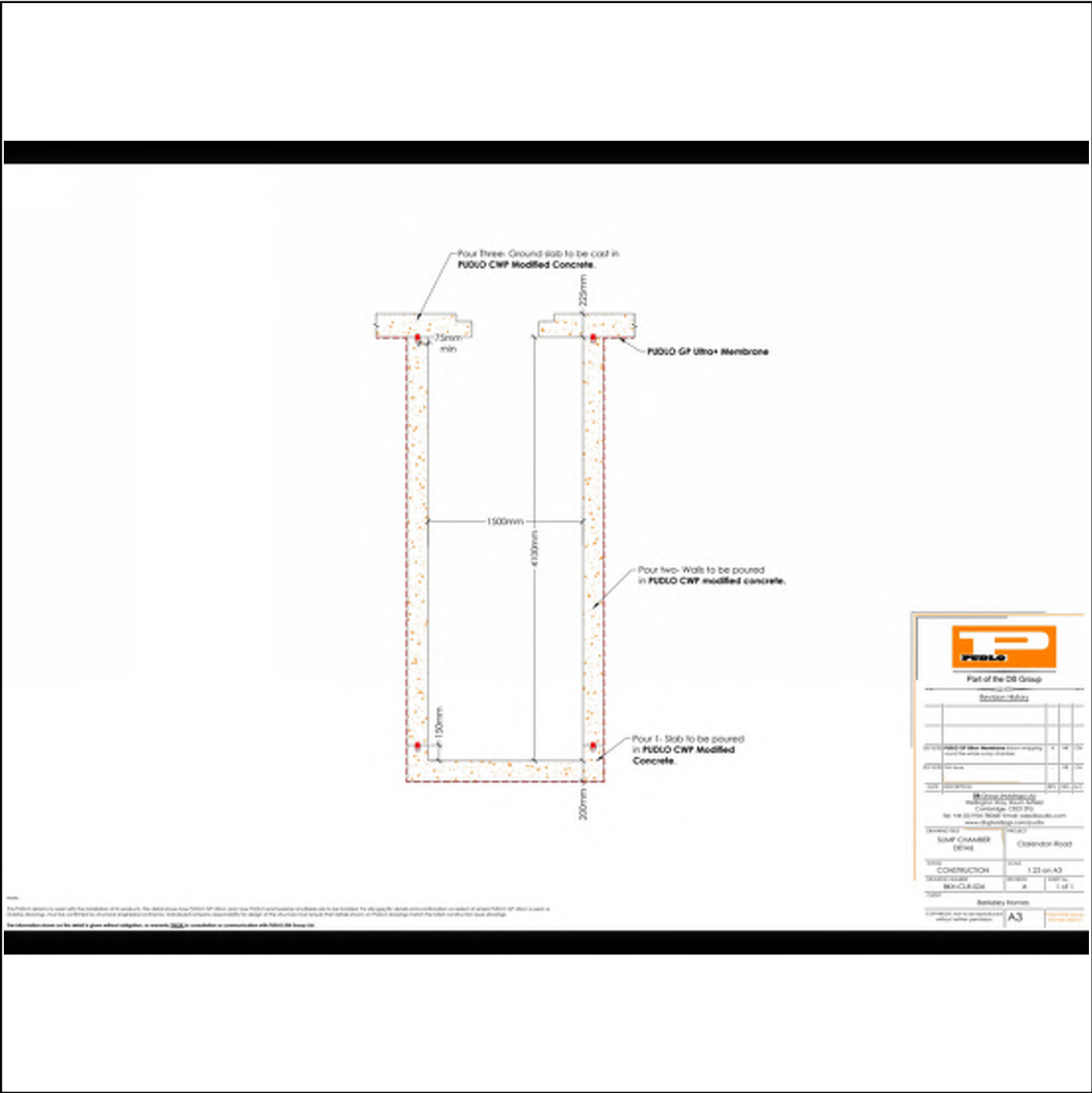
Sump Chamber Detail
