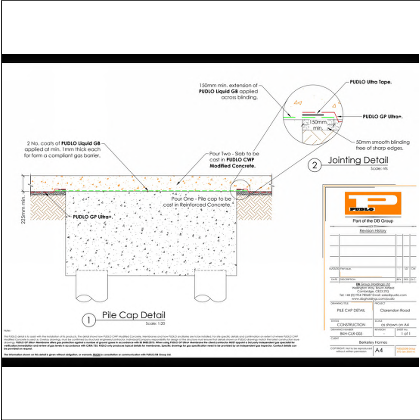
Pile Cap Detail
