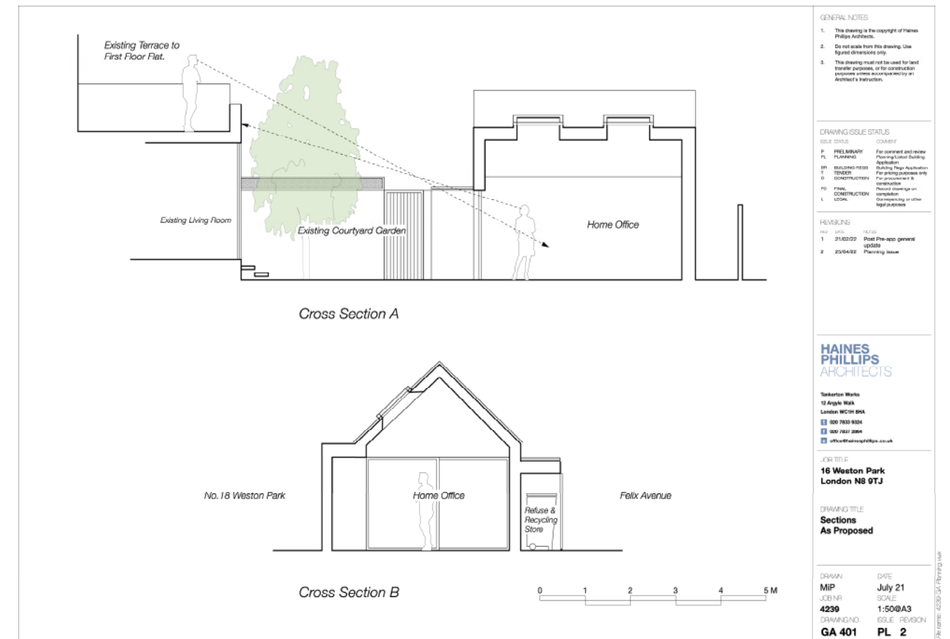
Consented proposed sections
