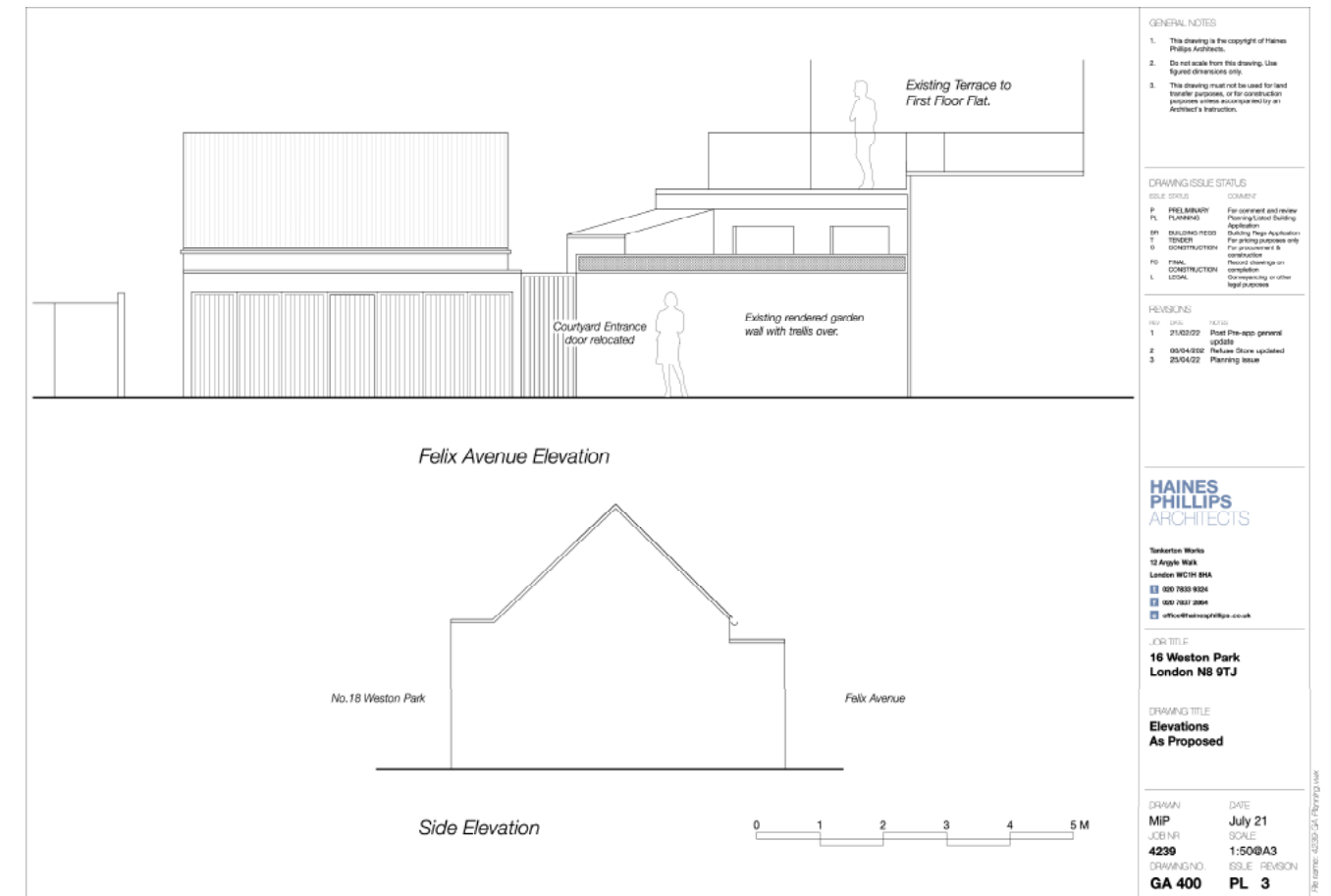
Consented proposed elevations
