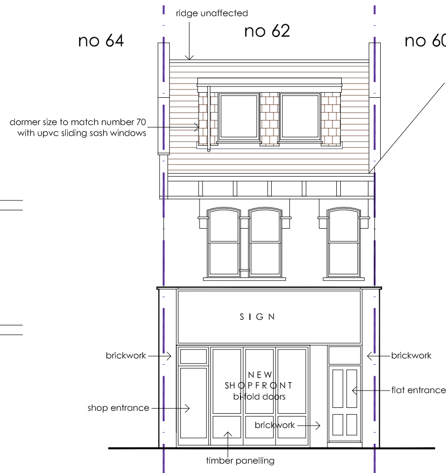
front elevation
