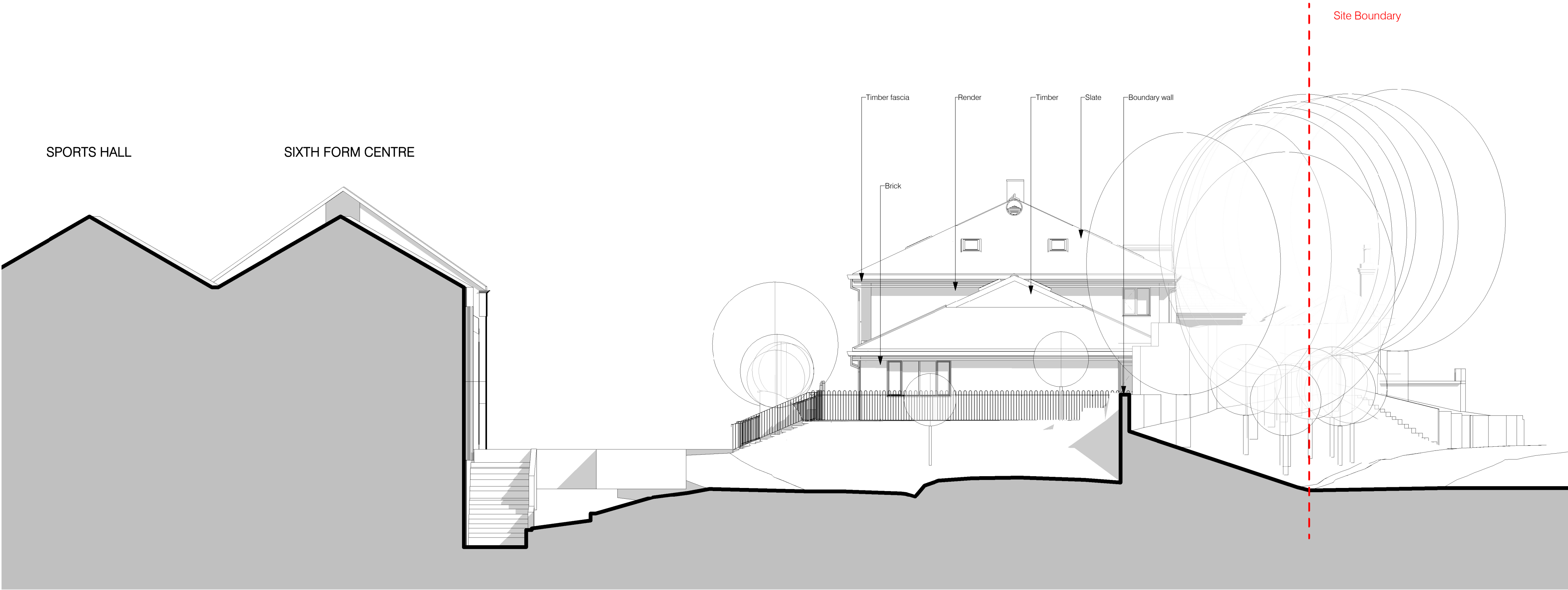
Existing - Elevation C 1 : 100
