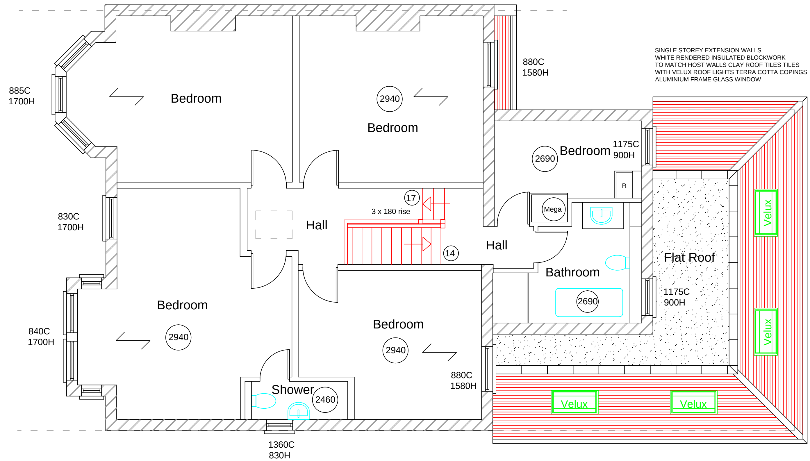
EXISTING FIRST FLOOR
