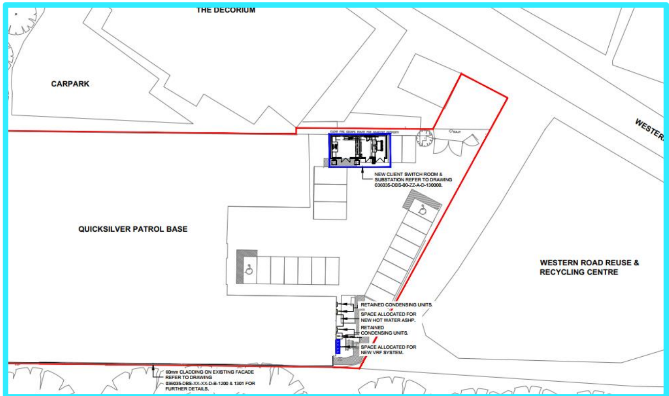
Figure 6.1: Site plan showing proposed plant layout.
