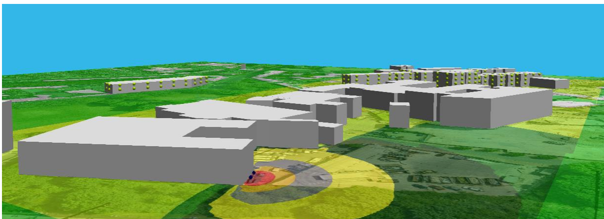
Figure 6.2: 3D Acoustic model with noise sources
