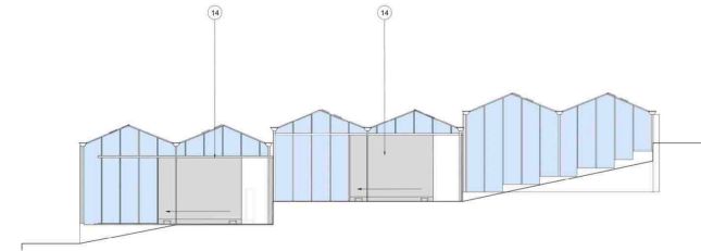
West Elevation
