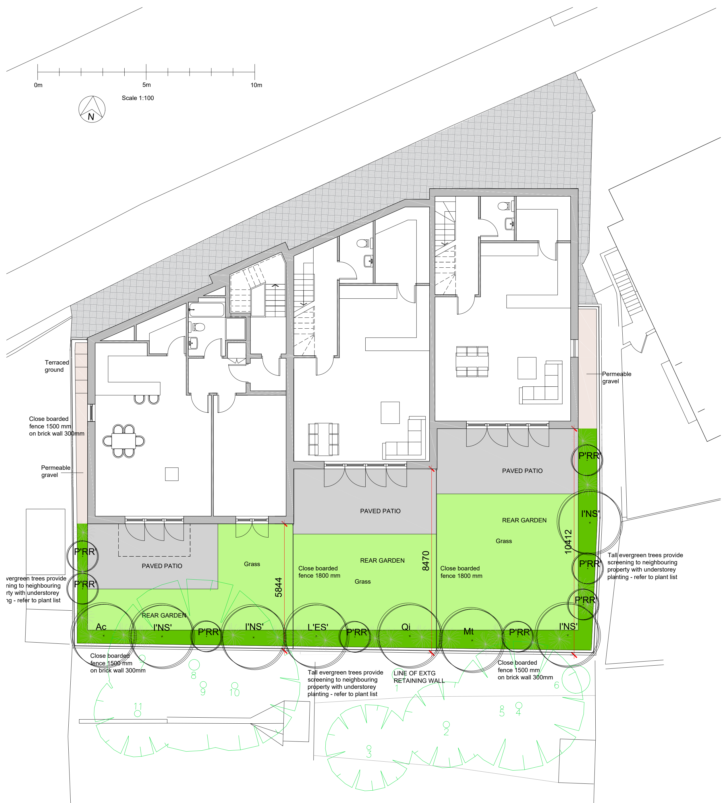
LOWER GROUND FLOOR LANDSCAPING PLAN
