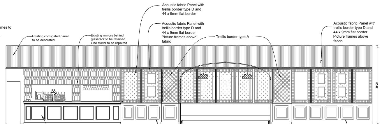
Elevation H
