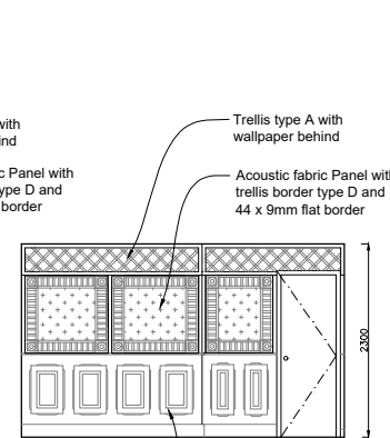
Elevation C
