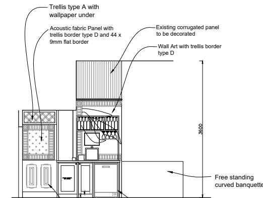
Elevation D
