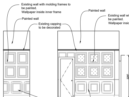
Elevation F
