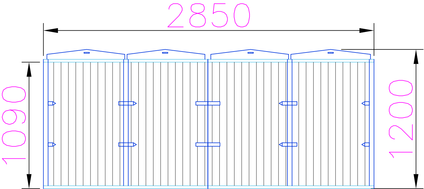
Front Elevation
