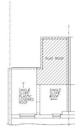
ROOF PLAN
