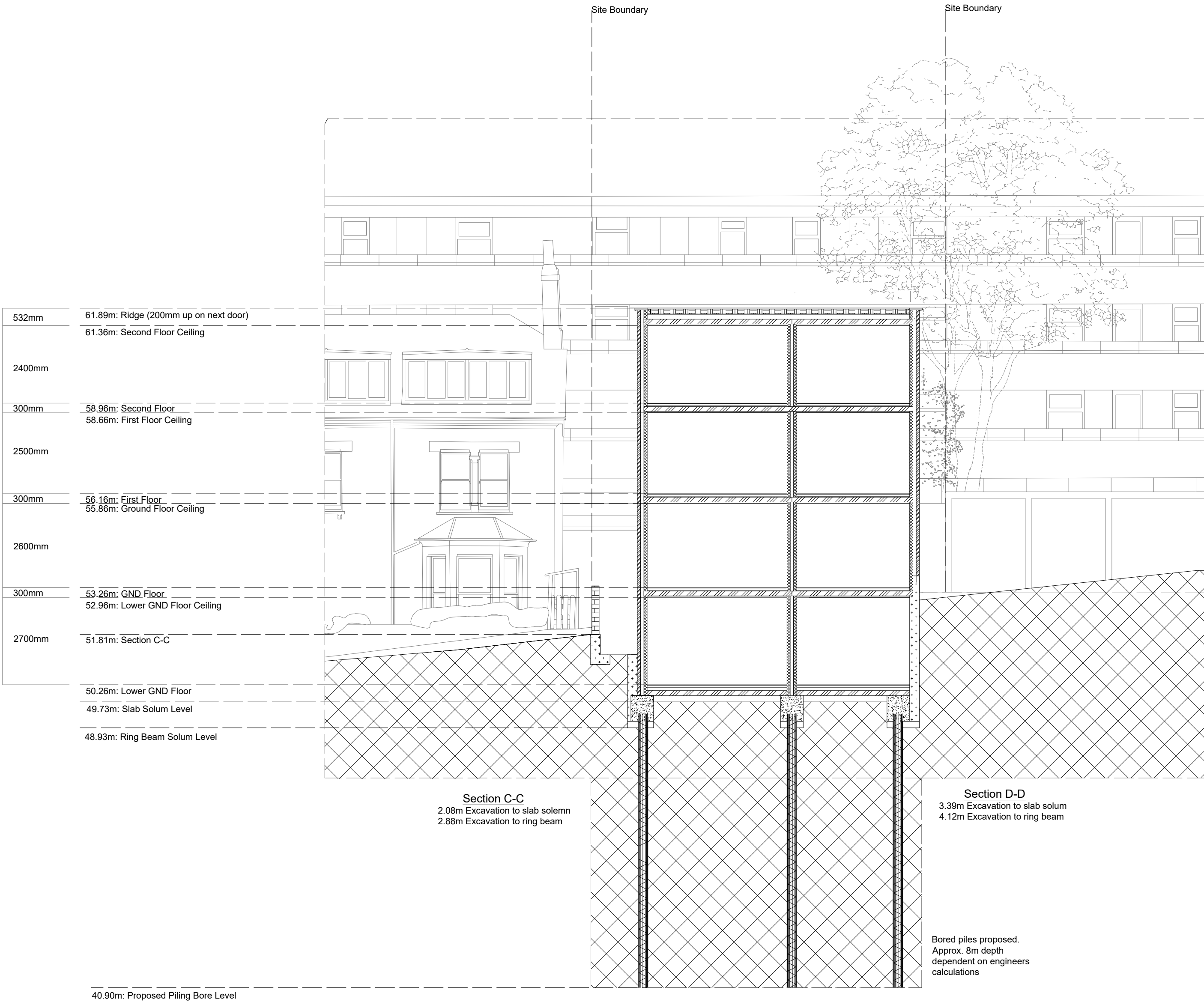
Transverse Section
