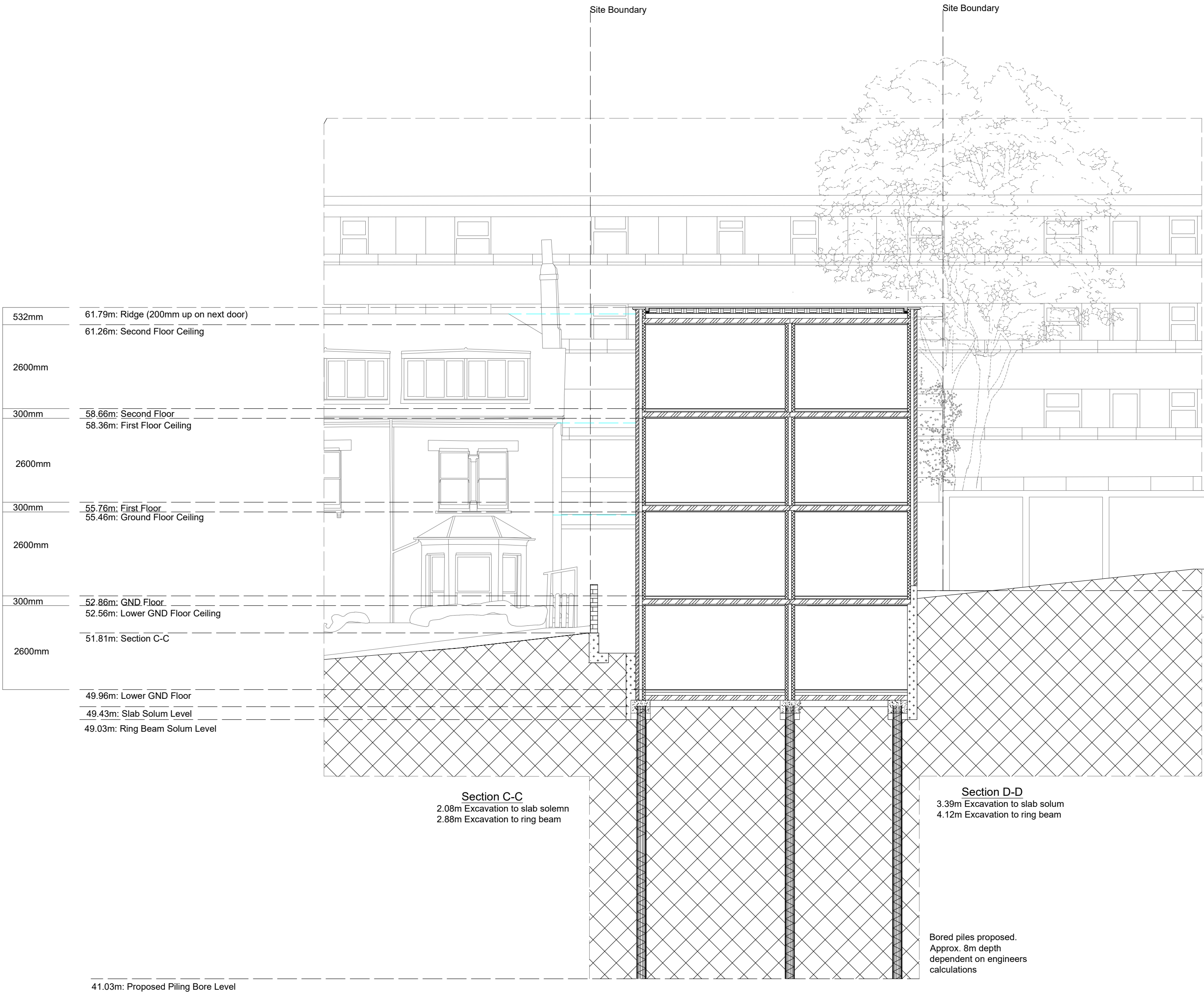
Transverse Section
