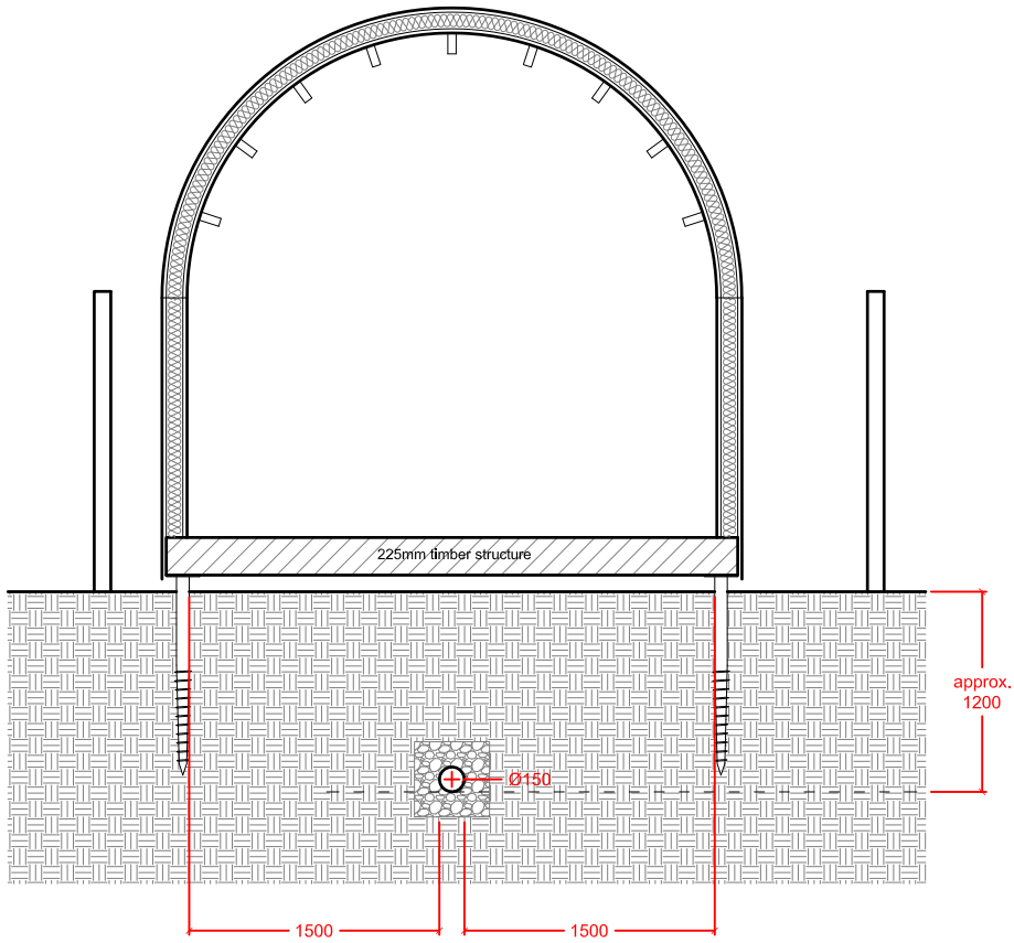
PIPE BRIDGING DETAIL - scale 1:50
