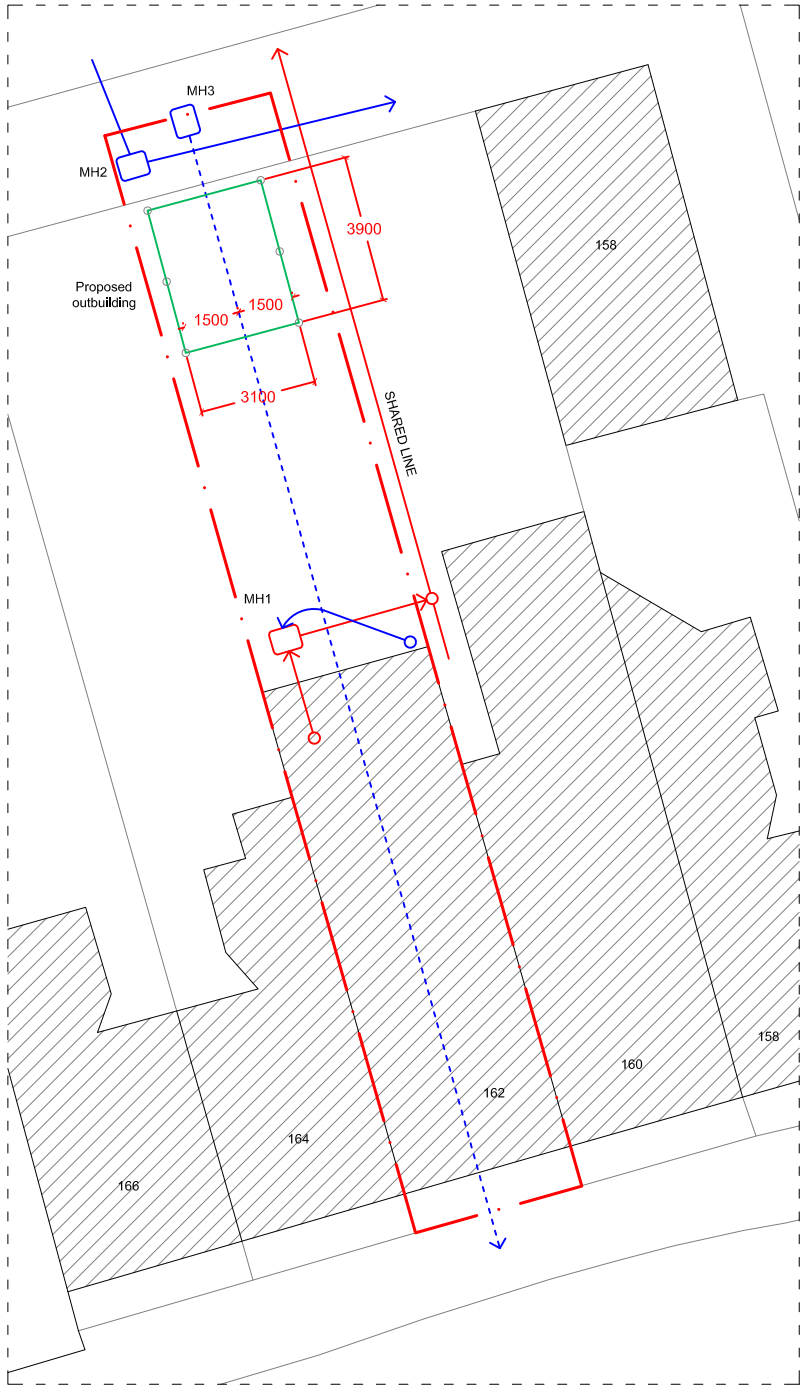
SEWER LAYOUT RELATIVE TO PROPOSED BUILDING - scale 1:200
