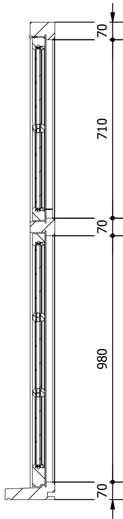
elevation section A-A ( 1 : 15 )
