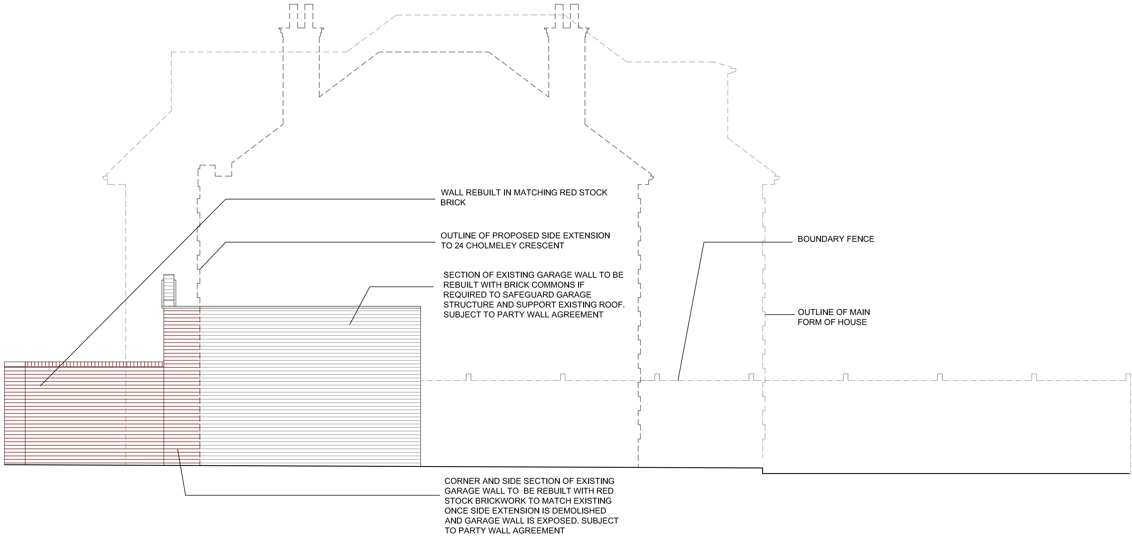
PROPOSED SECTION F - SIDE GARAGE WALL
