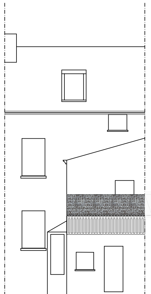
REAR ELEVATION AS EXISTING
