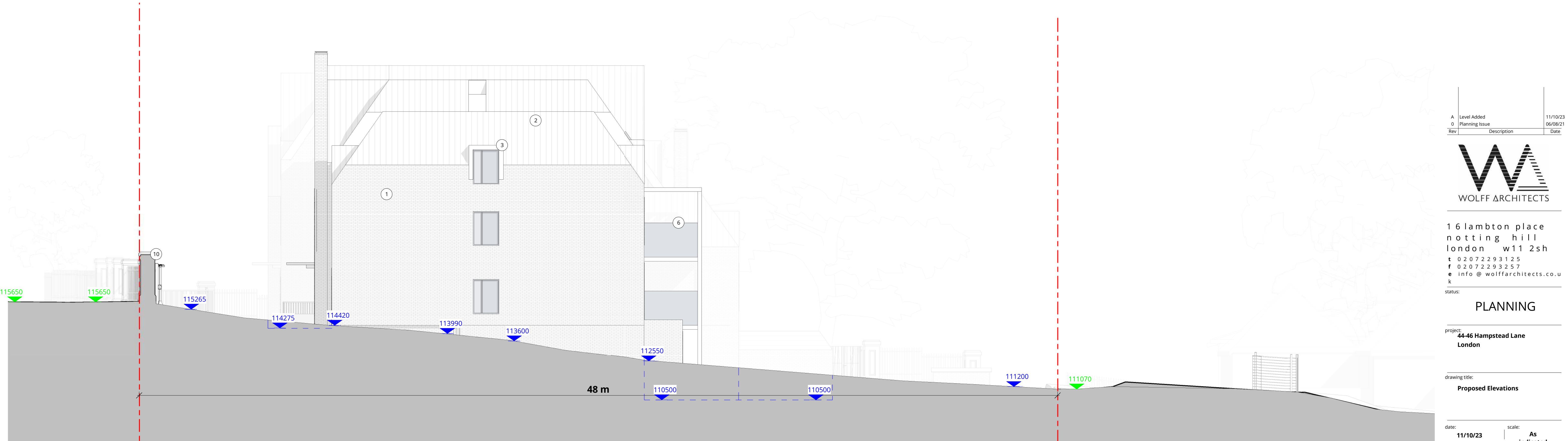
Proposed Eastern Elevation 1:100
