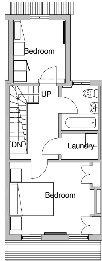
Proposed First Floor 1 : 100
